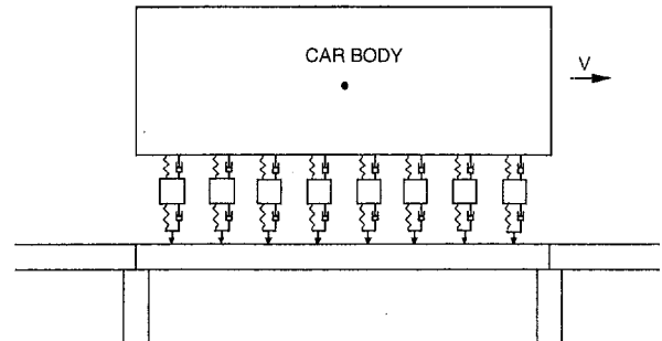
Fig. 2 Model of single car supported with multiple magnets and traveling along a guideway
