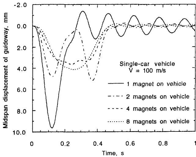
Fig. 3 Midspan displacement of guideway for single car with various magnets traveling along guideway at 100 m/s (360 km/h)
