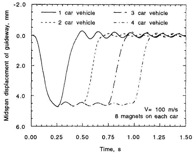
Fig. 5 Midspan displacements of guideway for multicar vehicles with eight magnets on each car traveling along guideway at 100 m/s (360 km/h)
