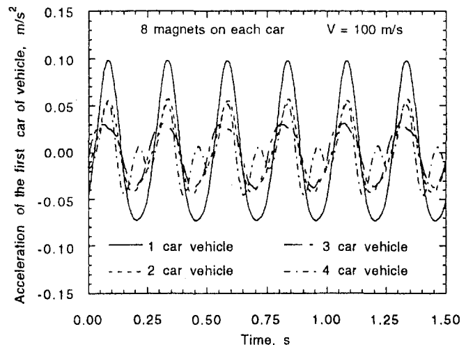
Fig. 6 Car body accelerations for multicar vehicles with eight magnets on each car traveling along guideway at 100 m/s (360 km/h)
