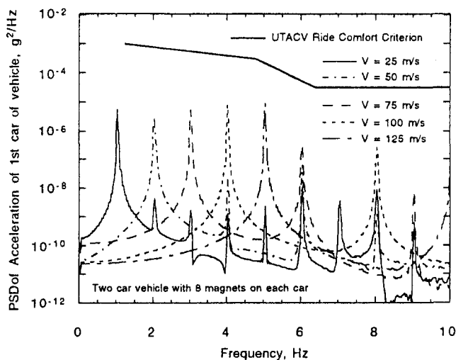
Fig. 8 PSD values of car-body accelerations for two-car vehicle with eight magnets on each car traveling along guideway at various speeds; UTACV Ride Comfort Criterion shown for comparison
