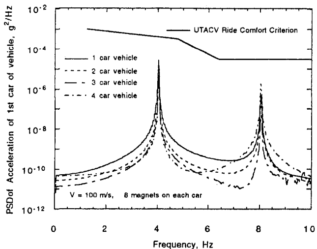
Fig. 7 PSD values of car-body accelerations for multicar vehicles with eight magnets on each car traveling along guideway at 100 m/s; UTACV Ride Comfort Criterion shown for comparison
