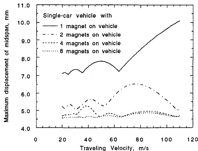
Fig. 4 Maximum midspan displacements of guideway for single car with various magnets traveling along guideway at various speeds
