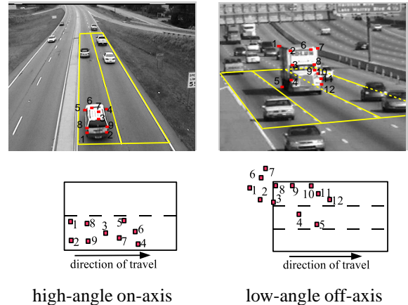
Figure 1: High-angle (left) versus low-angle (right) scenarios compared. In the later, a single homography is not sufficient, because a vehicle may map to multiple lanes.
