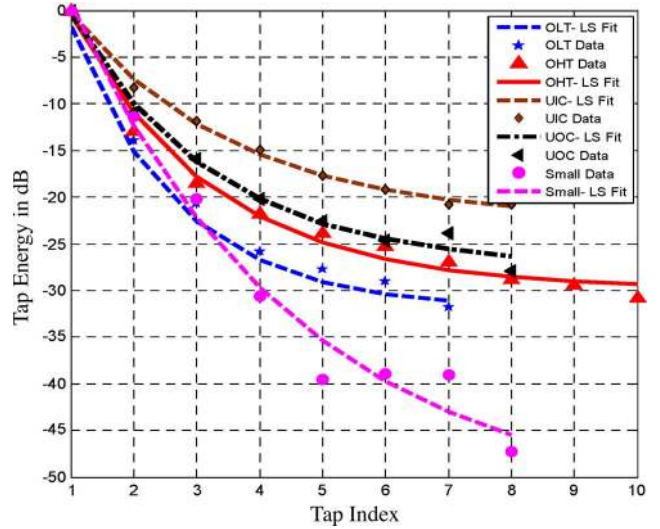
Fig. 7. Averaged tap energies with LS fits for all regions for a 5-MHz bandwidth.
