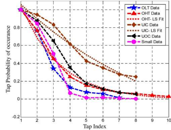
Fig. 6. Steady-state tap probability for state 1 (P[tap “on”]) versus tap index for all regions for a 5-MHz bandwidth.
