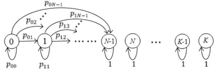
Fig. 8: Markov chain for X_n when K > N .
