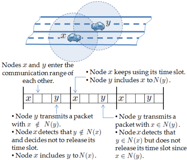
Fig. 5: The SRP condition preventing node x from unnecessarily releasing its time slot.
