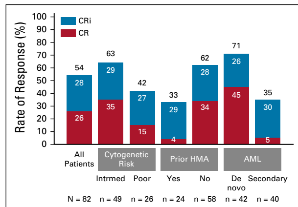
FIG 1. Complete remission (CR)/CR with incomplete blood count recovery (CRi) rates by patient subgroups. The graph shows the rates of CR and CRi in all patients, as well as key patient subgroups sorted by baseline characteristics. The numbers in the bars represent the percentage of patients with a given response, and the black number at the top of each bar is the total CR/CRi percentage in a given subgroup. Partial remissions are not shown, because only one patient had a partial remission. AML, acute myeloid leukemia; HMA, hypomethylating agent; intrmed, intermediate.
