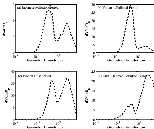
Figure 3. Mean aerosol volume distributions during four periods of observation during the ACE-Asia field campaign.
