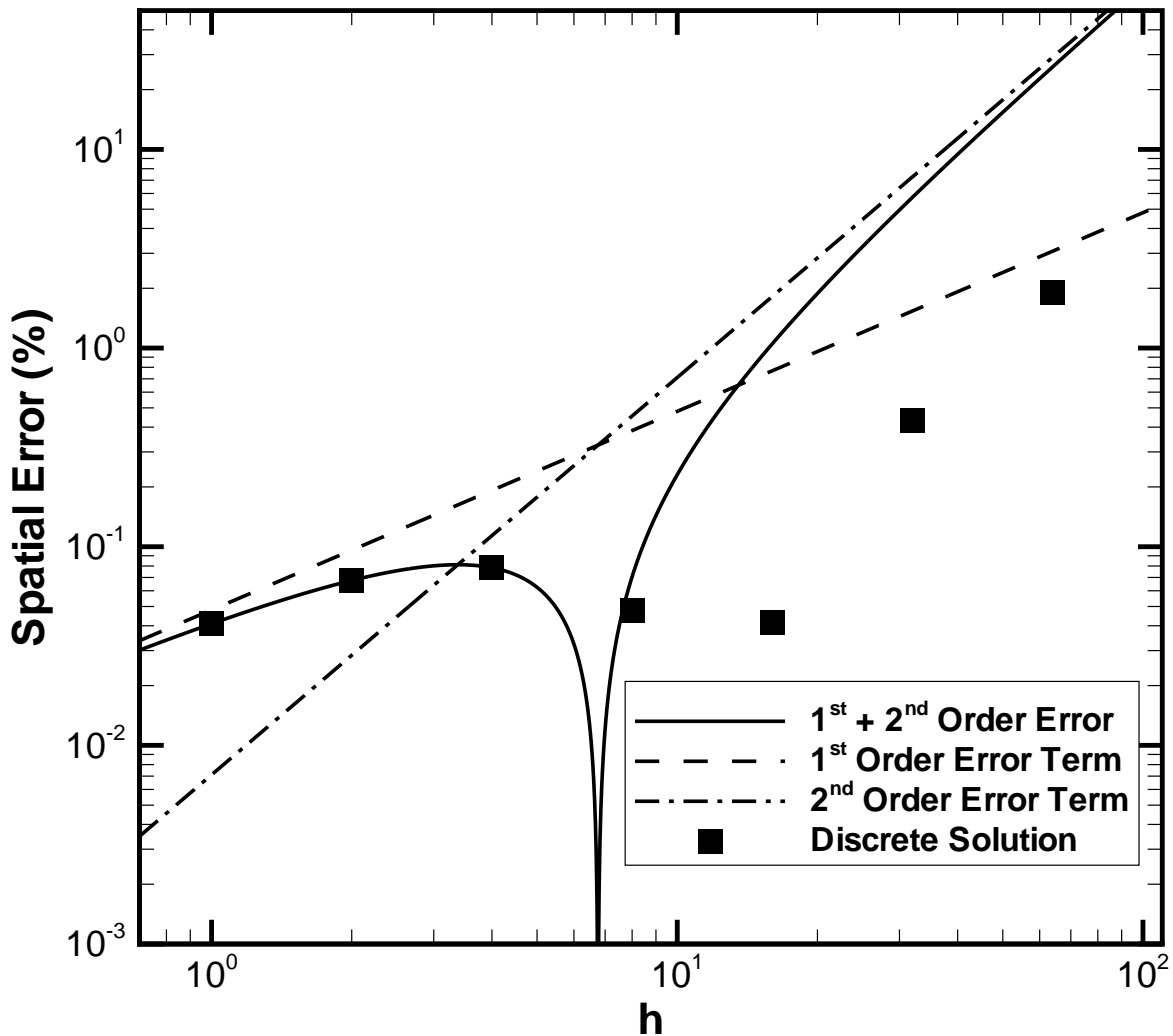
Figure 5. Demonstration of extrapolated error estimation for mixed first and second order schemes [286].
