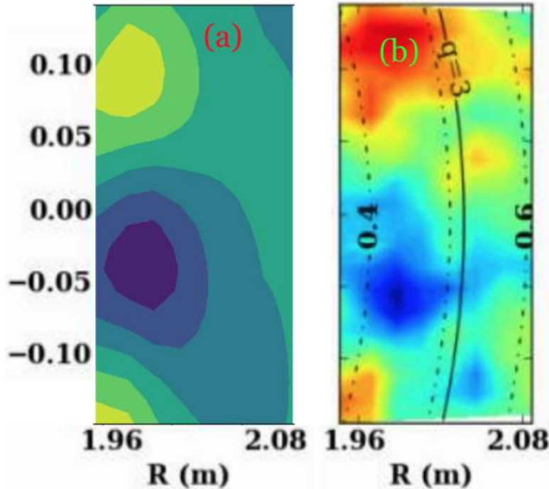
Figure 12. Comparison of n = 4 RSAE mode GTC simulation data and experimental ECEI data for DIII-D #159243 at 807.3 ms. 2D structure on a poloidal plane of \delta T_e / T_{e0} for (a) GTC simulation data, after being processed through the Synthetic-Diagnostic-Platform, and (b) experimental ECEI data.
