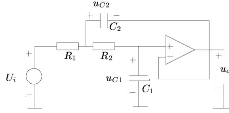
Fig. 2. A low-pass filter.
