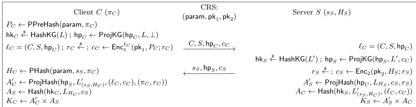
Fig. 2. Generic two-round VPAKE Construction
