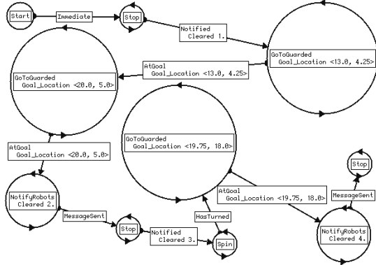
Figure 5: MissionLab FSA for Robot1
