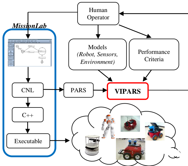
Figure 1: Verification System Architecture
