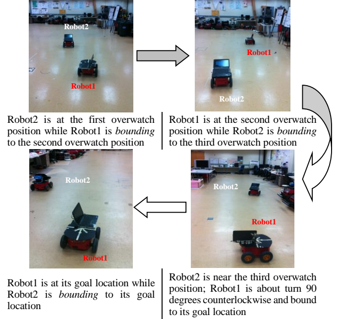
Figure 8: Snapshots of the Bounding Overwatch Mission
