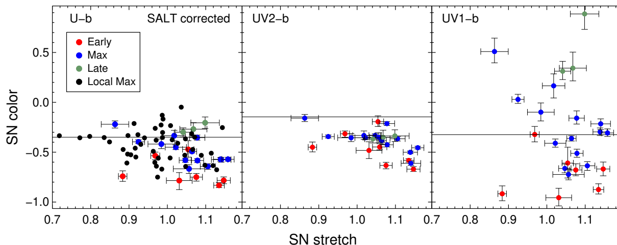
Fig. 10.— Various SN Ia stretch-color relations, with colors measured directly from the SALT color law corrected Keck spectra. The colors shown are U - b , UV1 - b and UV2 - b – see Fig. 3 for filter definitions. SNe are color-coded according to the phase of the spectrum as defined in Fig. 1. The black points in the U - b distribution refers to the U - b distribution of local SNe Ia at maximum light from local SN surveys (e.g. Jha et al. 2006). The error-bars for the SNLS SNe include propagated uncertainties from host galaxy subtraction (§ 3.3).
