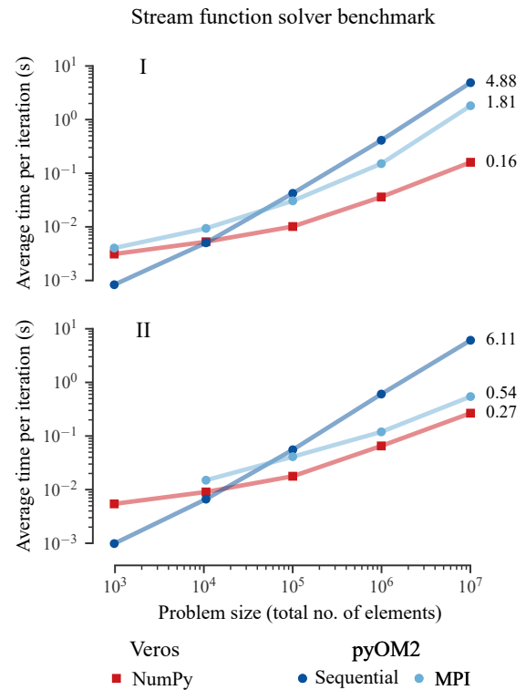
Figure 2. Thanks to pyAMG’s AMG preconditioner, the Veros stream function solver is between 2 (24 CPUs, II) and 11 (4 CPUs, I) times faster than pyOM2’s parallel conjugate gradient solver for large problem sizes.
