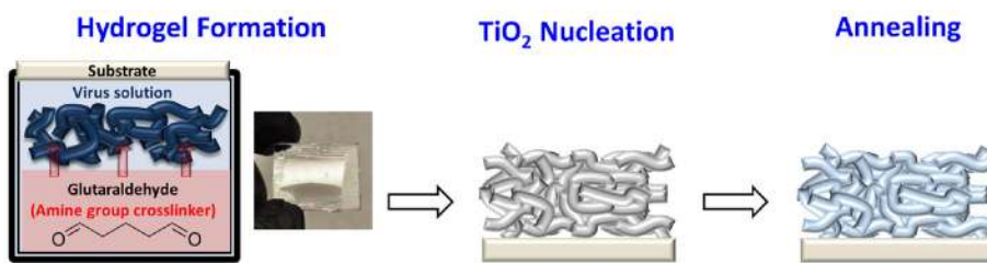
Figure 1. Schematic illustration of 3D porous TiO 2 photoanode fabrication process, including (1) hydrogel formation, (2) TiO 2 nucleation and (3) annealing.
