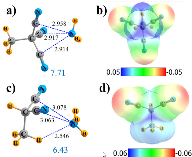
Figure 3. Geometries and monomer MEP of complex of NH 3 with H 3 C-C(CN) 3 (a,b) and H 3 C-CH(CN) 2 (c,d).
