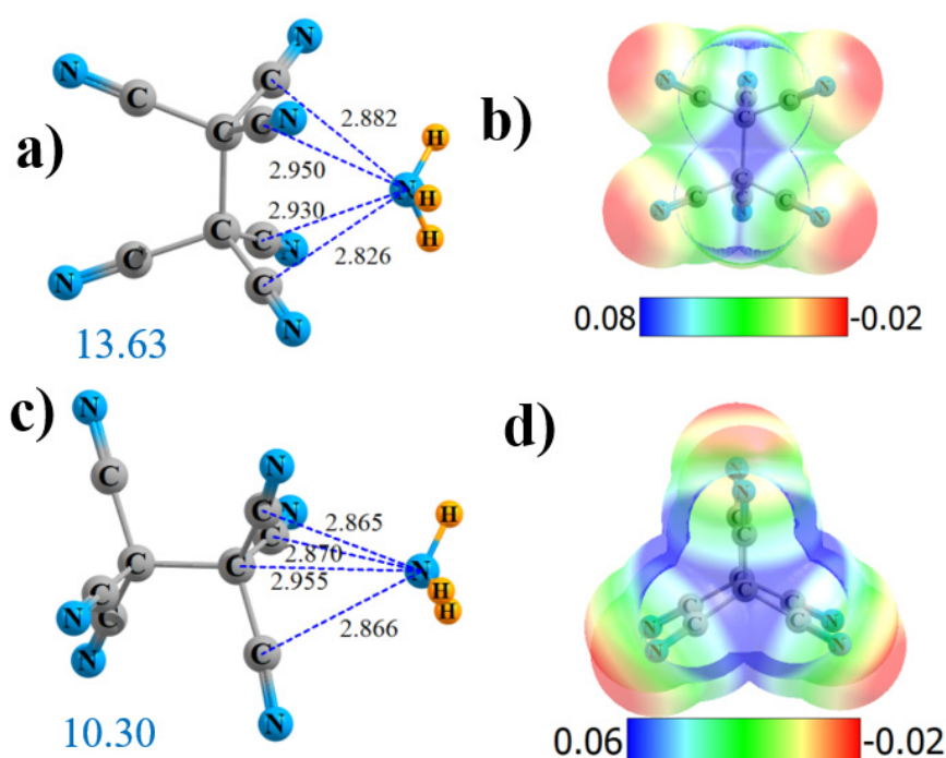
Figure 1. Geometries and monomer molecular electrostatic potential (MEP) of (\text{CN})_3\text{C}-\text{C}(\text{CN})_3 interacting with \text{NH}_3 from the side (a,b) and end (c,d). Dotted lines denote AIM bond paths. Large blue numbers indicate interaction energy in kcal/mol. Distances in Å and MEP in au. MEP can be converted to kcal/mol by factor of 627.51.
