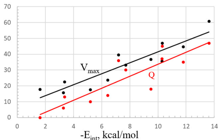
Figure 7. Linear fitting of the interaction energy to the MEP maximum (kcal/mol, black) and total charge transfer Q (red, me).
