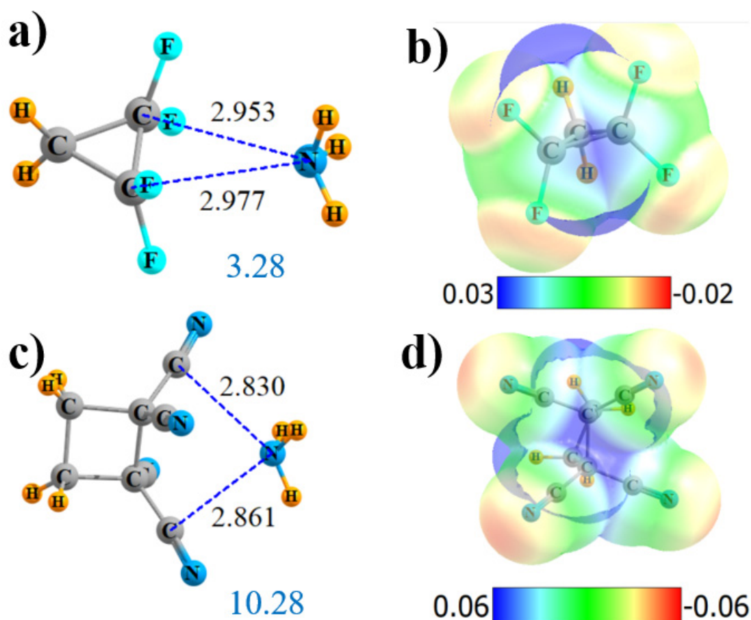
Figure 6. Geometries and monomer MEP of the complex of NH 3 with cyclic Lewis acids CH 2 {CF 2 } 2 (a,b) and CH 2 CH 2 {C(CN) 2 } 2 (c,d).
