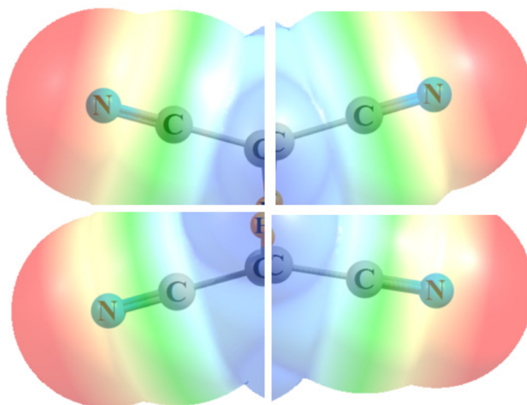
Figure 8. Partial MEP of \text{MeC}\equiv\text{N} in four different orientations, pieced together so as to compare with the MEP of (\text{CN})_2\text{HC}-\text{CH}(\text{CN})_2 in Figure 2b.
