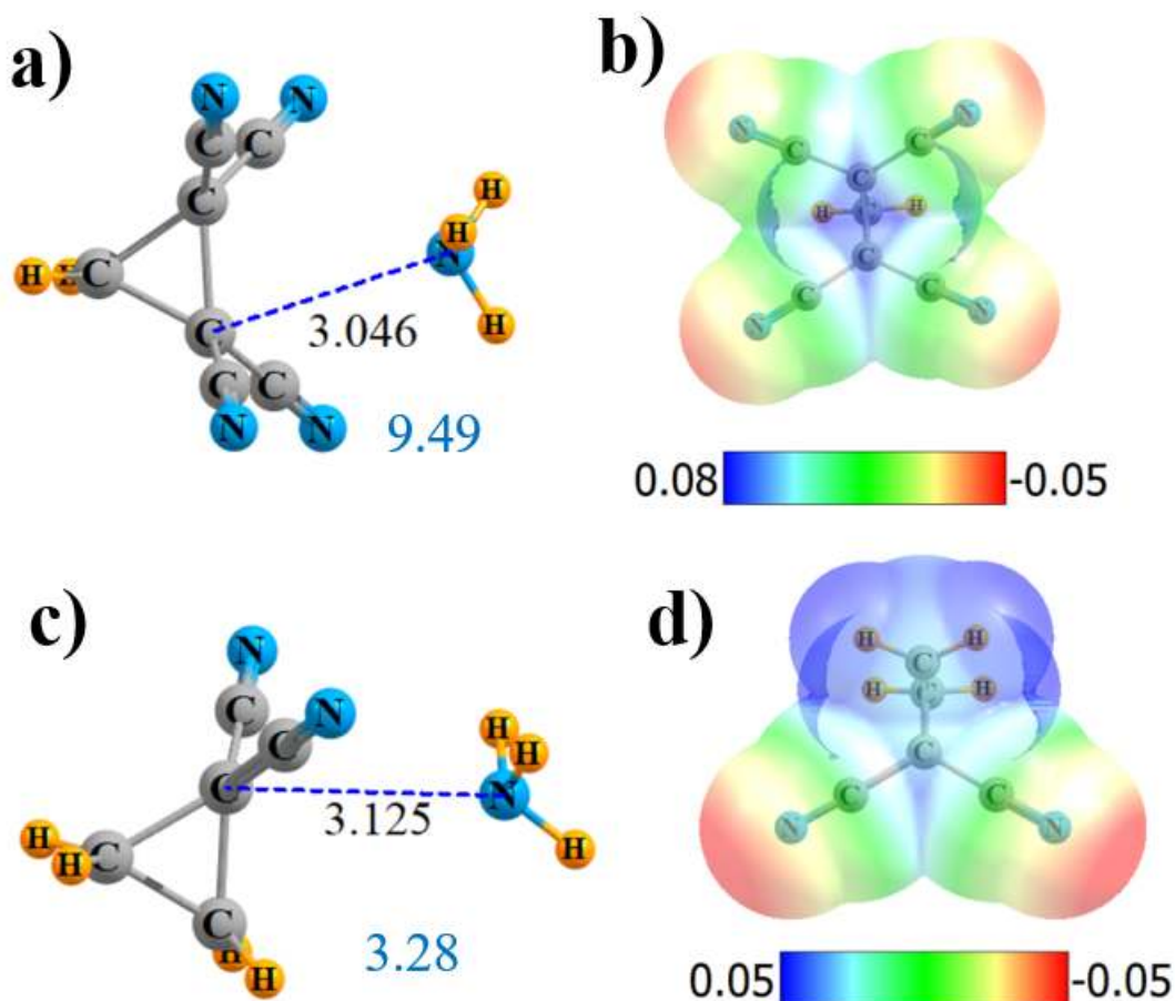
Figure 5. Geometries and monomer MEP of the complex of \text{NH}_3 with cyclic Lewis acids \text{CH}_2[\text{C}(\text{CN})_2]_2 (a,b) and \text{CH}_2\text{CH}_2\text{C}(\text{CN})_2 (c,d).
