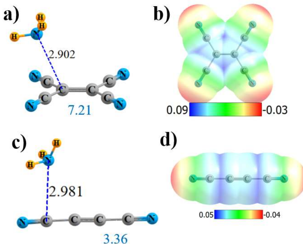
Figure 4. Geometries and monomer MEP of the complex of \text{NH}_3 with (\text{CN})_2\text{C}=\text{C}(\text{CN})_2 (a,b) and (\text{CN})\text{C}\equiv\text{C}(\text{CN}) (c,d).
