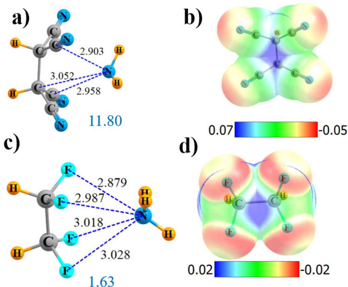
Figure 2. Geometries and monomer MEP of complex of \text{NH}_3 with (\text{CN})_2\text{HC}-\text{CH}(\text{CN})_2 (a,b) and \text{F}_2\text{HC}-\text{CHF}_2 (c,d).
