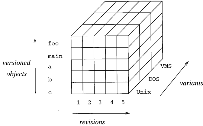
Figure 11. Product versioning.
