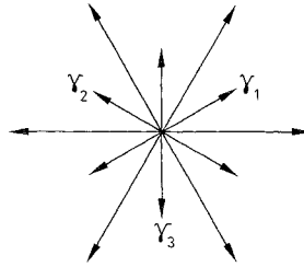
Fig. 2. The root of diagram for G_2
