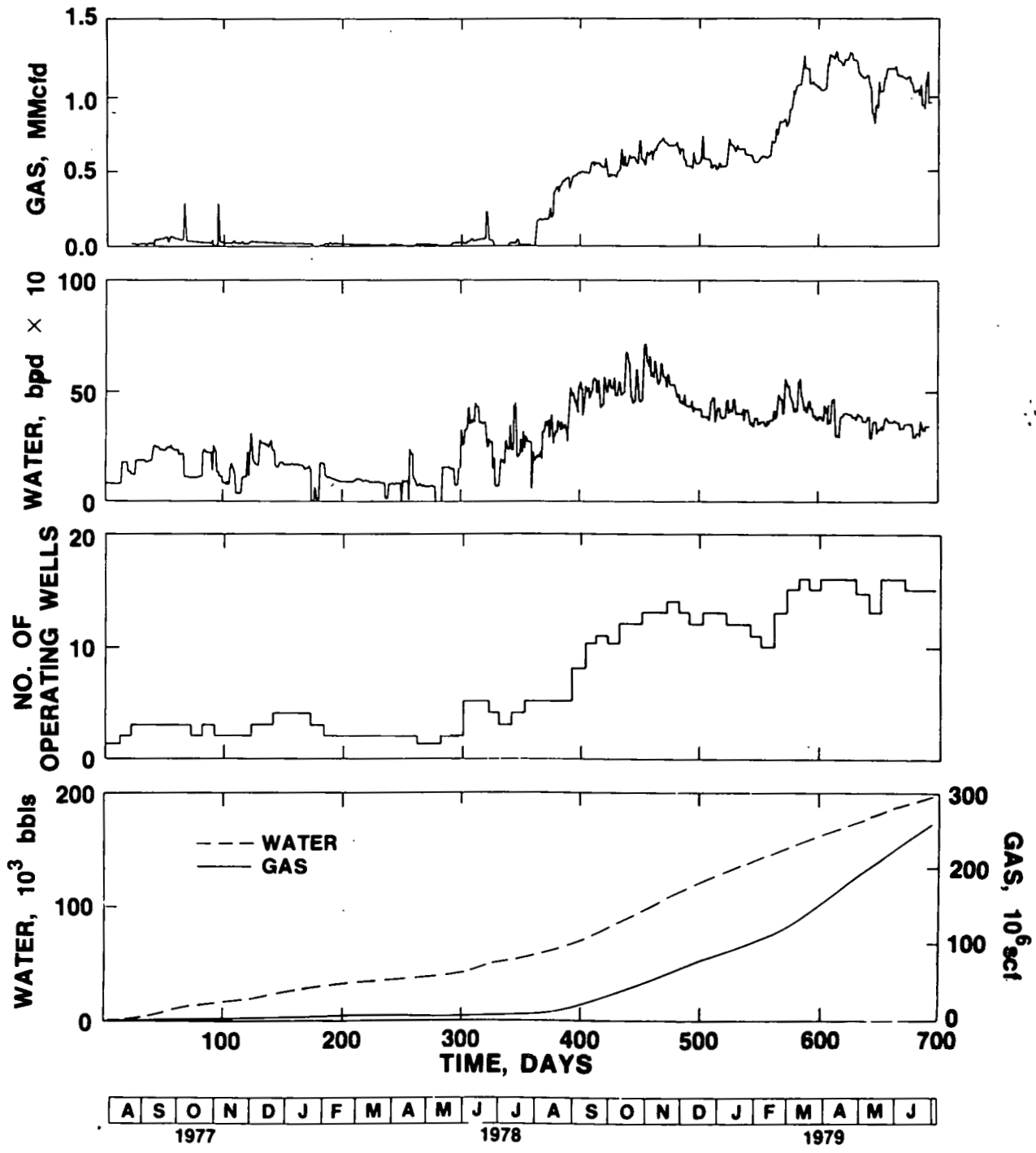
FIGURE 56 - DAILY PRODUCTION; NUMBER OF OPERATING WELLS AND CUMULATIVE TOTAL AMOUNT OF GAS AND WATER PRODUCED FROM THE MARY LEE COAL BED DEGASIFICATION PATTERN NEAR OAK GROVE, JEFFERSON COUNTY, ALABAMA
