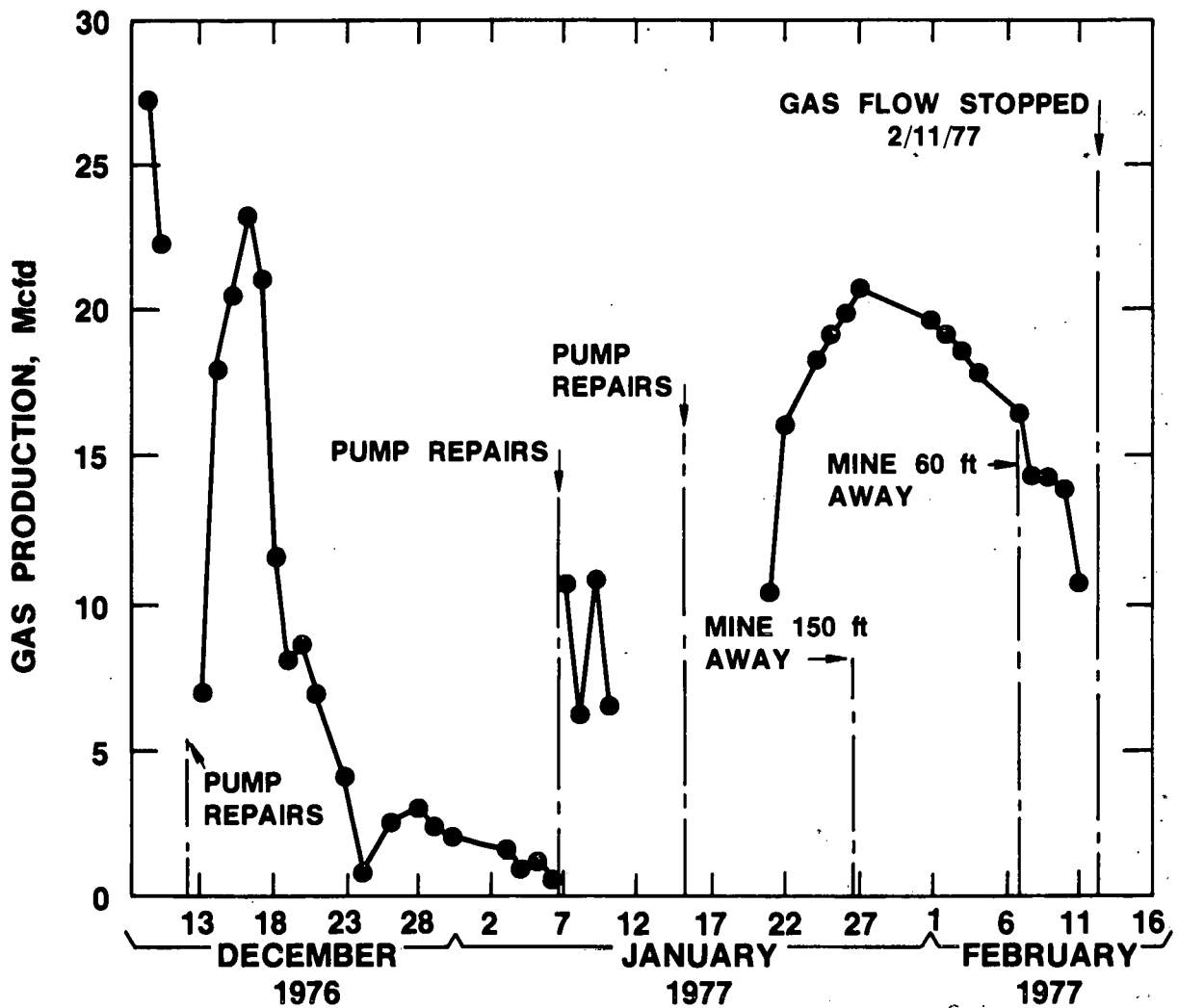
FIGURE 25. - DAILY GAS PRODUCTION FROM TW2, MARY LEE COALBED (23).
