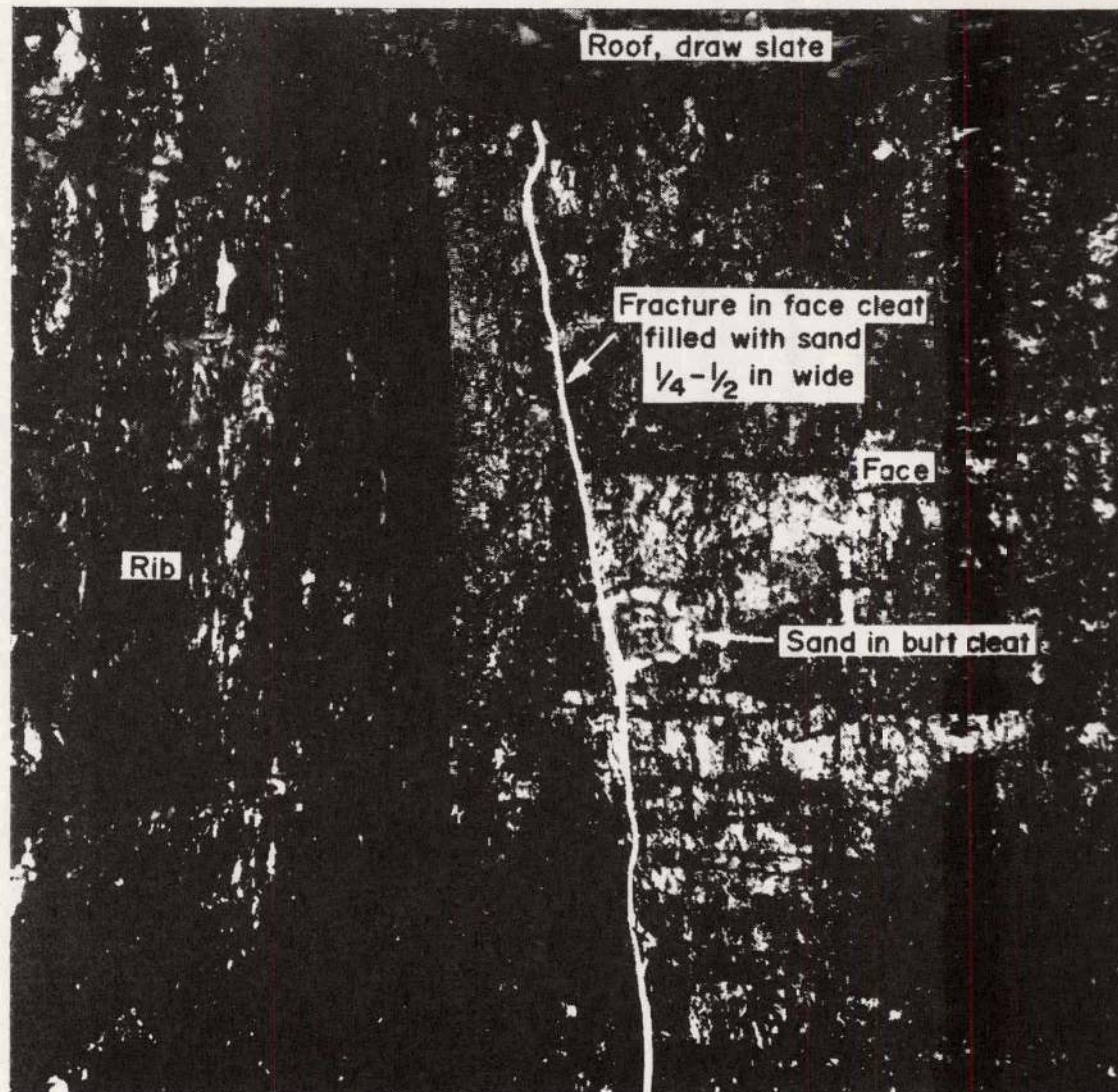
FIGURE 29. - INDUCED FRACTURE IN FACE CLEAT OF PITTSBURGH COALBED. NOTE TERMINATION OF FRACTURE AT DRAW SLATE (16).
