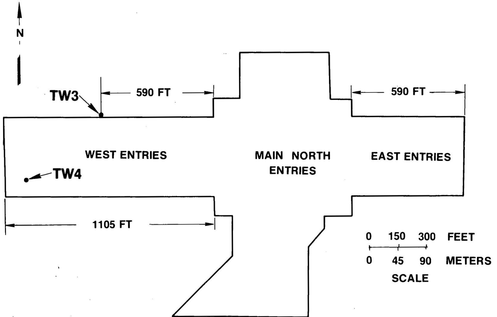
FIGURE 65. - VIEW OF MINE SHOWING TEST WELL LOCATIONS AND MINE ENTRIES STUDIED FOR GAS EMISSIONS.
