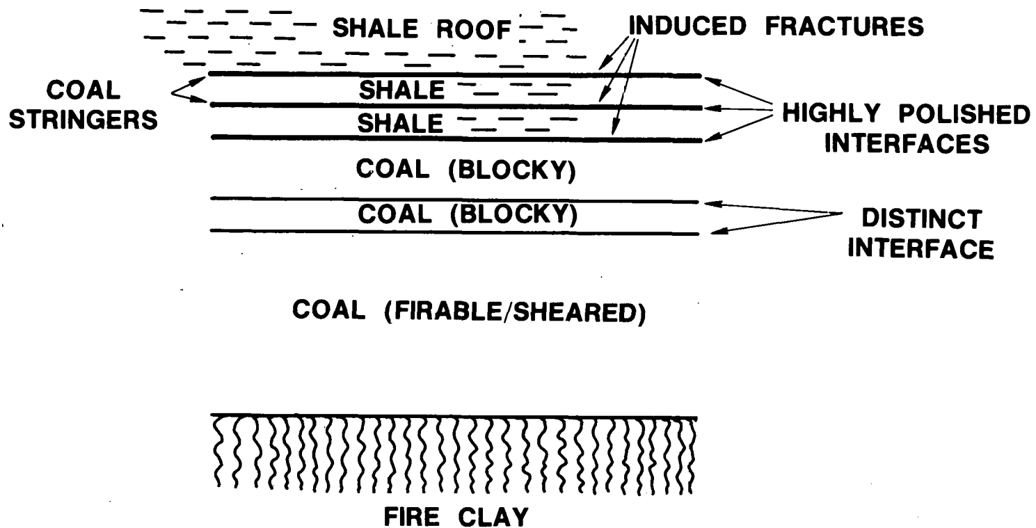
FIGURE 64. - SKETCH SHOWING POSITION AND ORIENTATION OF INDUCED FRACTURES FROM TW5 (HORIZONTAL PENETRATIONS)
