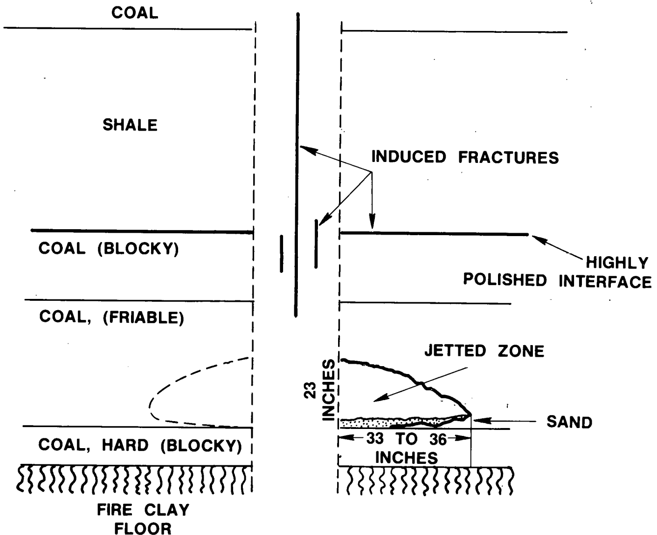
FIGURE 63. - SKETCH OF TW5 WELLBORE SHOWING POSITION AND ORIENTATION OF INDUCED FRACTURES AS INDICATED BY THE PRESENCE OF FLUORESCENT MATERIAL CONTAINED IN THE STIMULATION TREATMENT FLUID.
