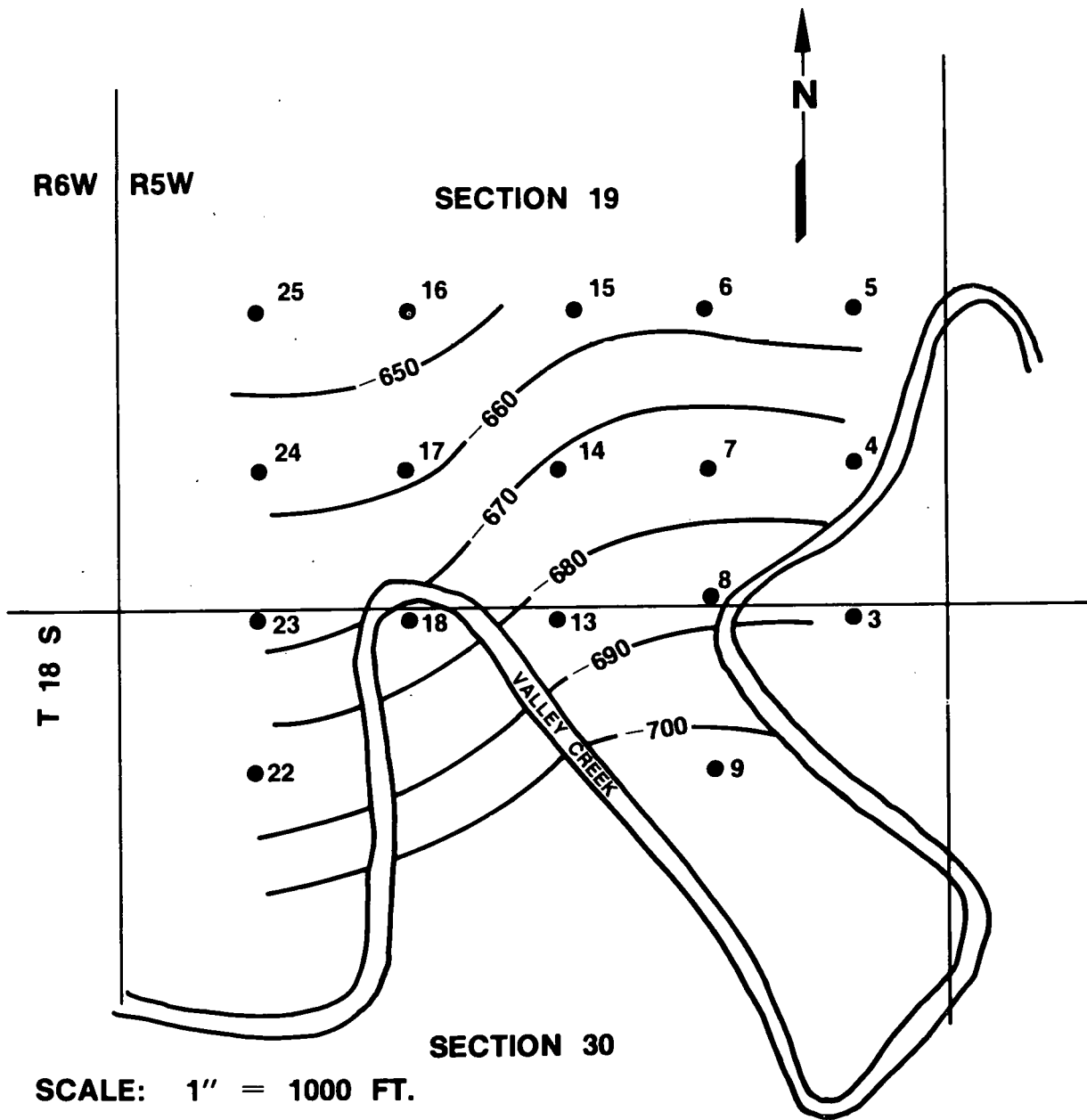
FIGURE 47. - OAK GROVE DEGASIFICATION GRID PATTERN, MARY LEE COALBED, JEFFERSON CO., ALABAMA
