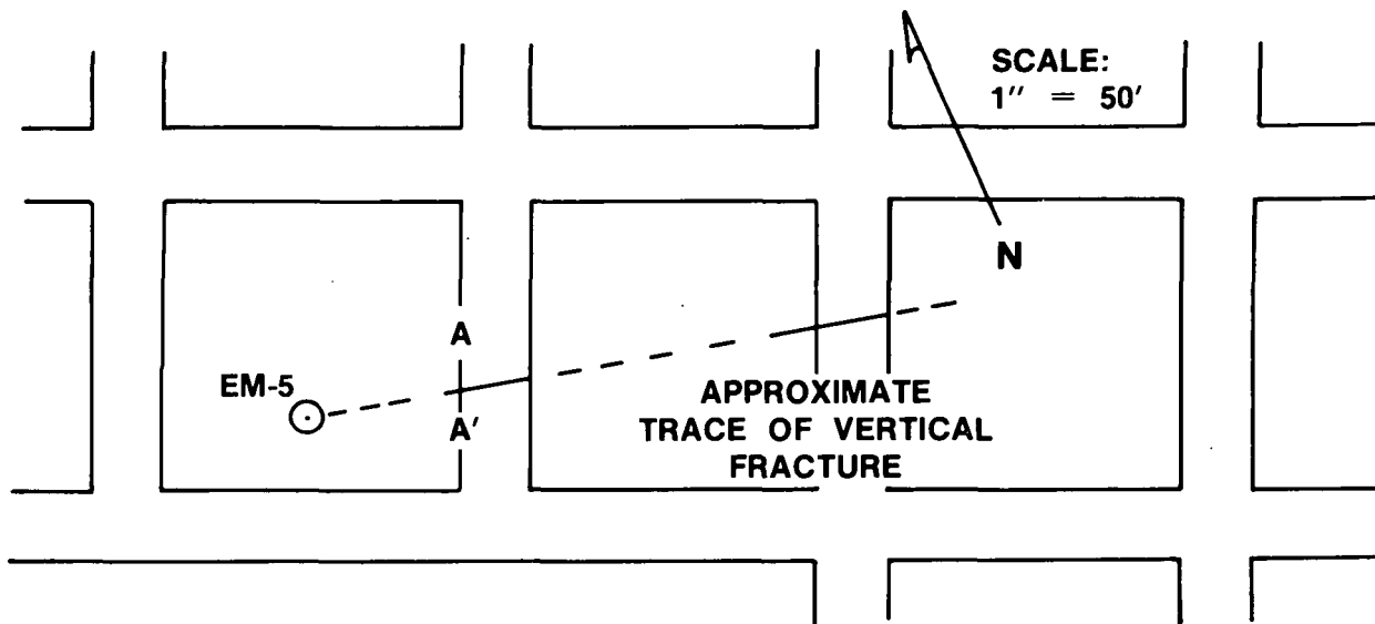
FIGURE 39. - POSITION AND ORIENTATION OF THE INDUCED FRACTURES OBSERVED NEAR DEGAS WELL NO. EM-5.
