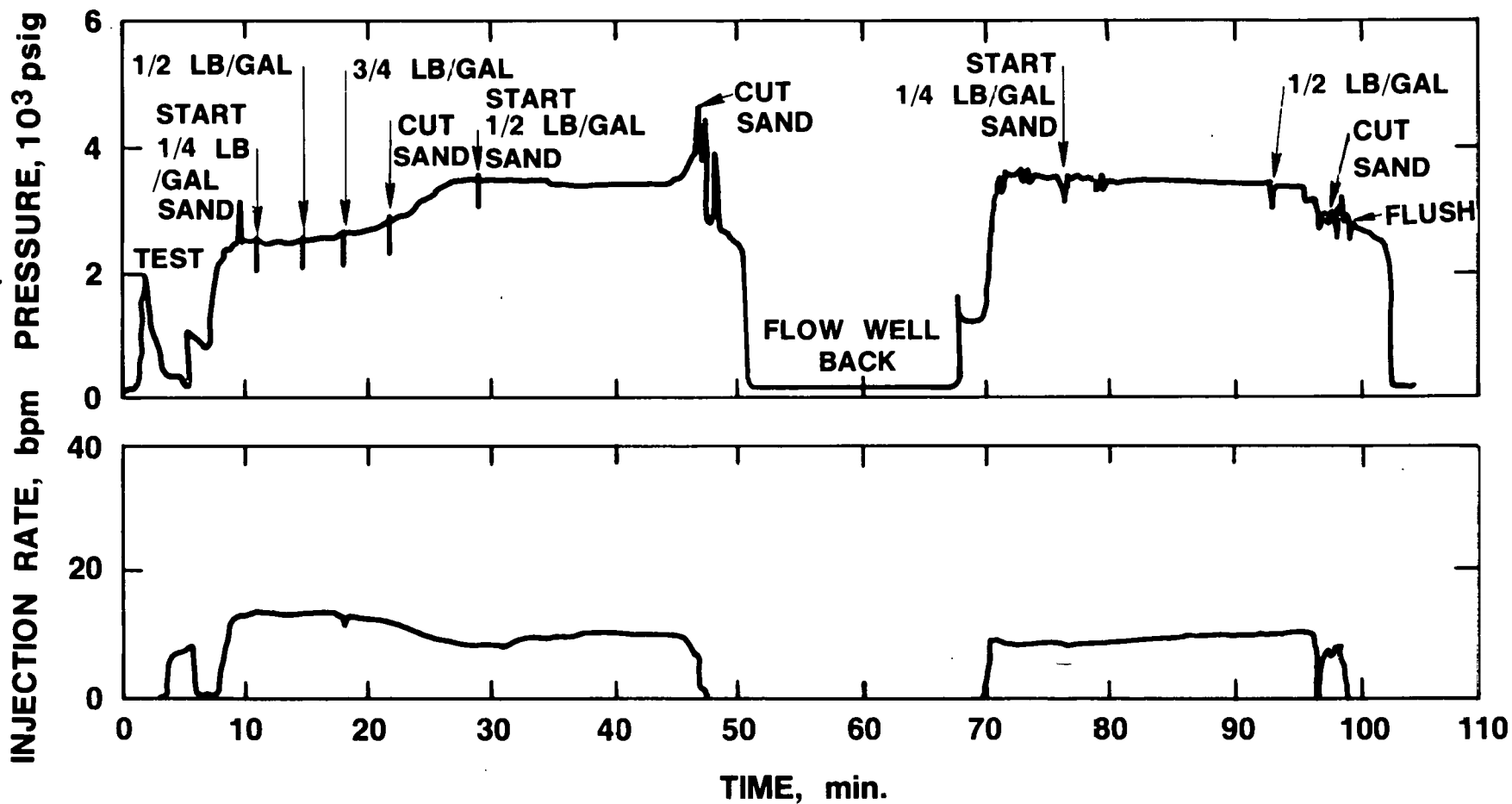
FIGURE 18. - WELL HEAD PRESSURE AND INJECTION RATE CHARTS OF HYDRAULIC STIMULATION TREATMENT OF POCAHONTAS NO. 3 COALBED (16).
