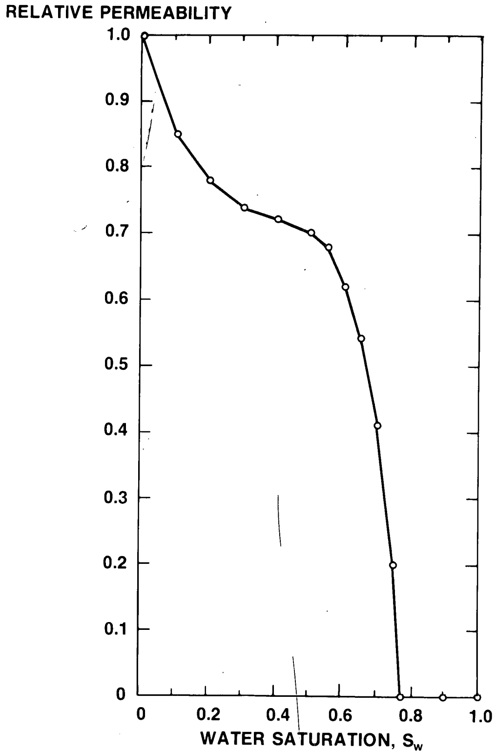
FIGURE 3. - GAS PERMEABILITY RELATIVE TO WATER SATURATION (22).
