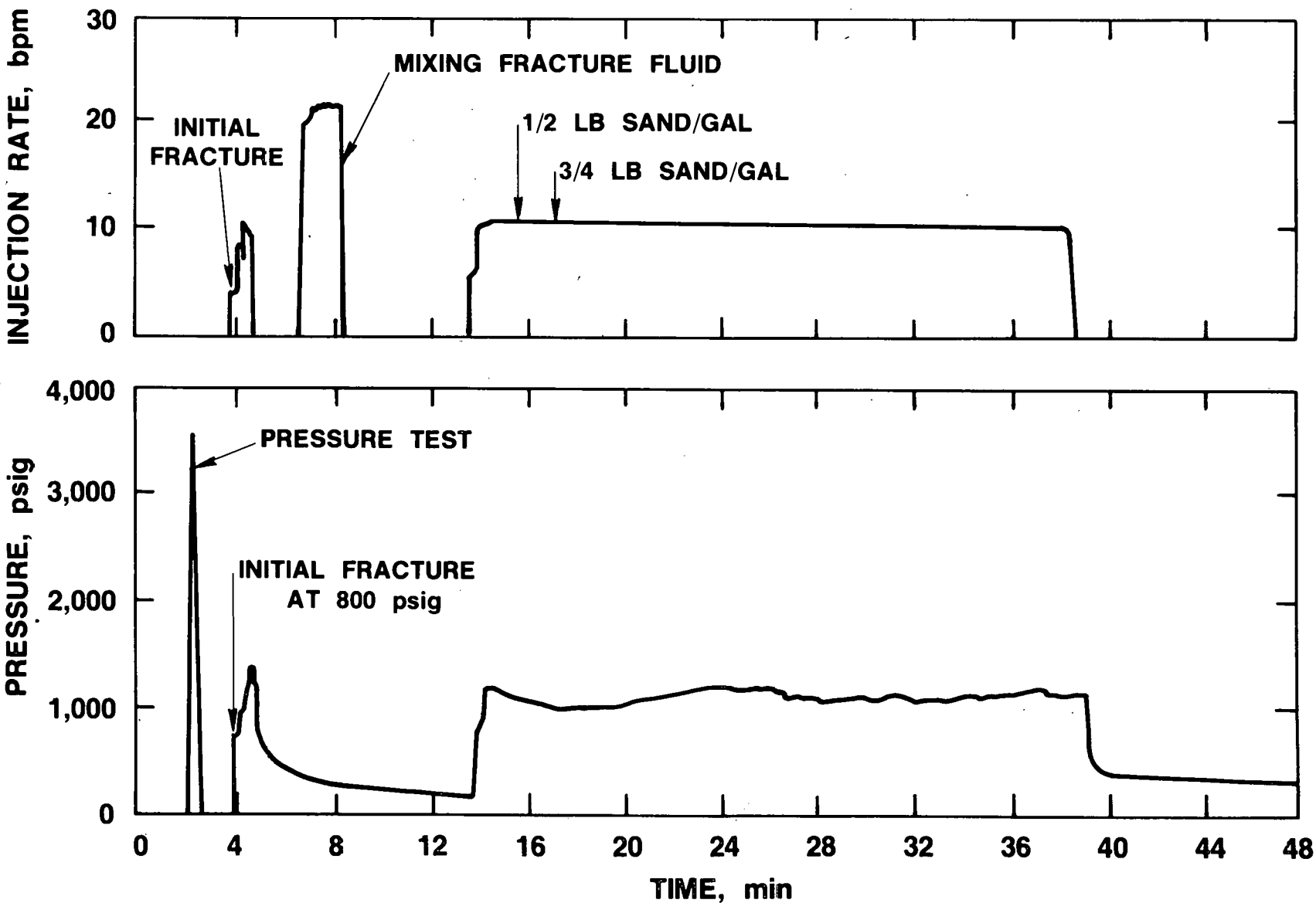
FIGURE 20. - WELLHEAD PRESSURE AND INJECTION RATE CHARTS OF HYDRAULIC STIMULATION OF THE MARY LEE COALBED (7).
