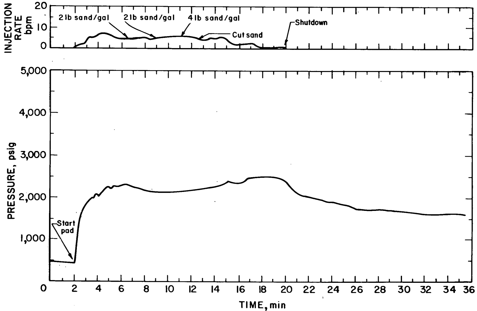
FIGURE 24. - HYDRAULIC STIMULATION PRESSURE AND FLUID INJECTION CHART TW2, MARY LEE COALBED (23).
