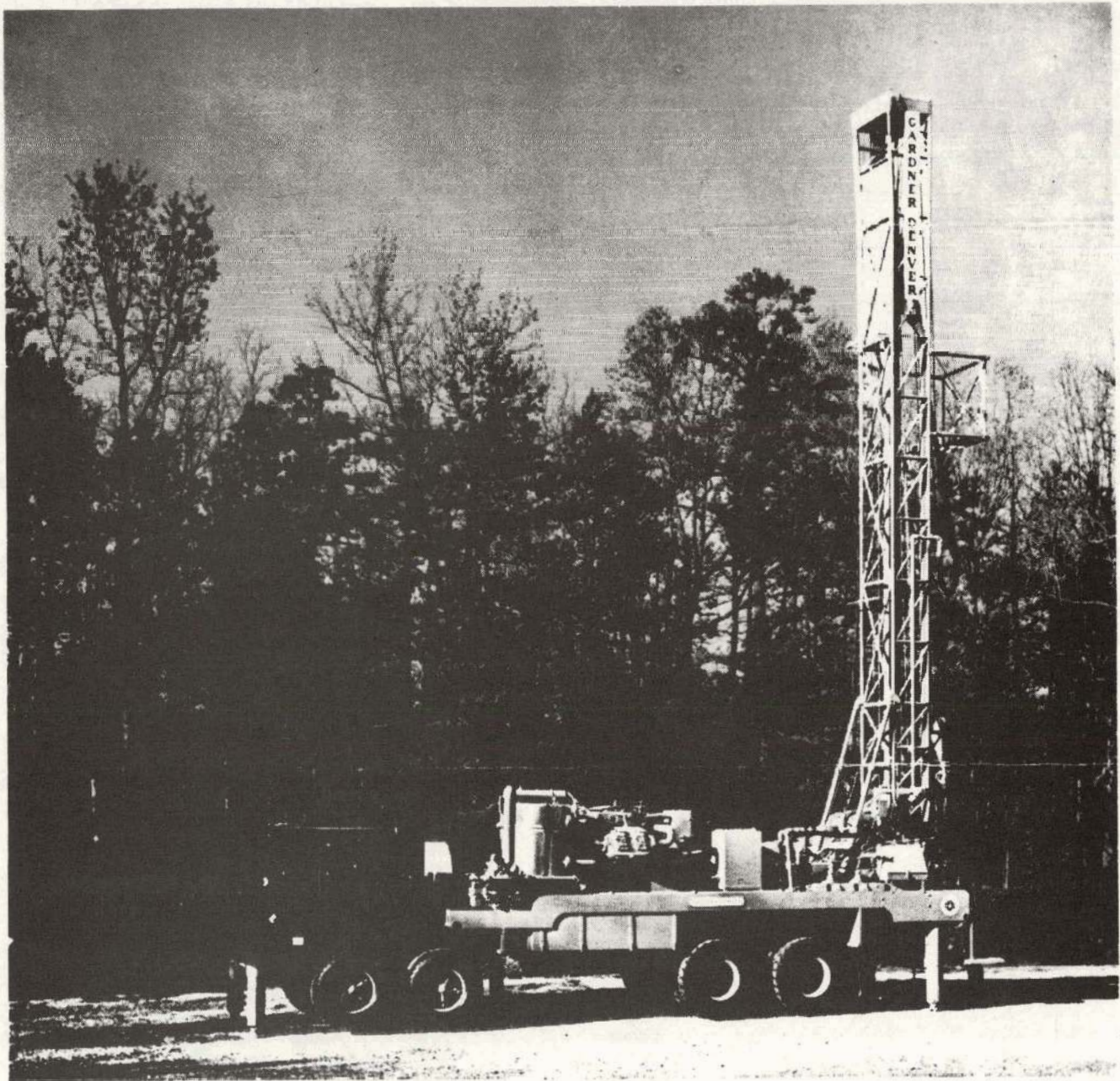
FIGURE 11. - TYPICAL SIZE AND TYPE OF DRILLING RIG USED TO ROTARY DRILL COALBED GAS DRAINAGE BOREHOLES.
