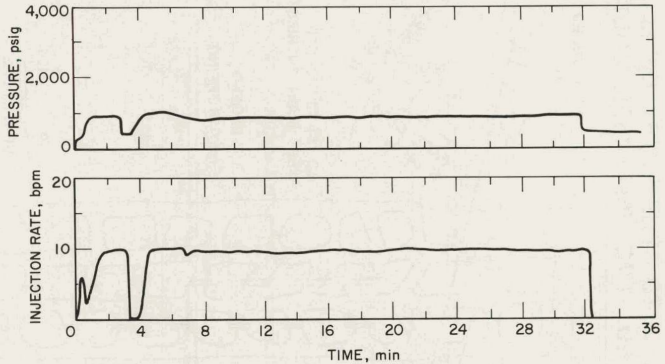
FIGURE 31. - PRESSURE AND INJECTION RATE CHARTS DURING HYDRAULIC STIMULATION, USBM NO.1 NE, JEFFERSON COUNTY, ILL. (16).
