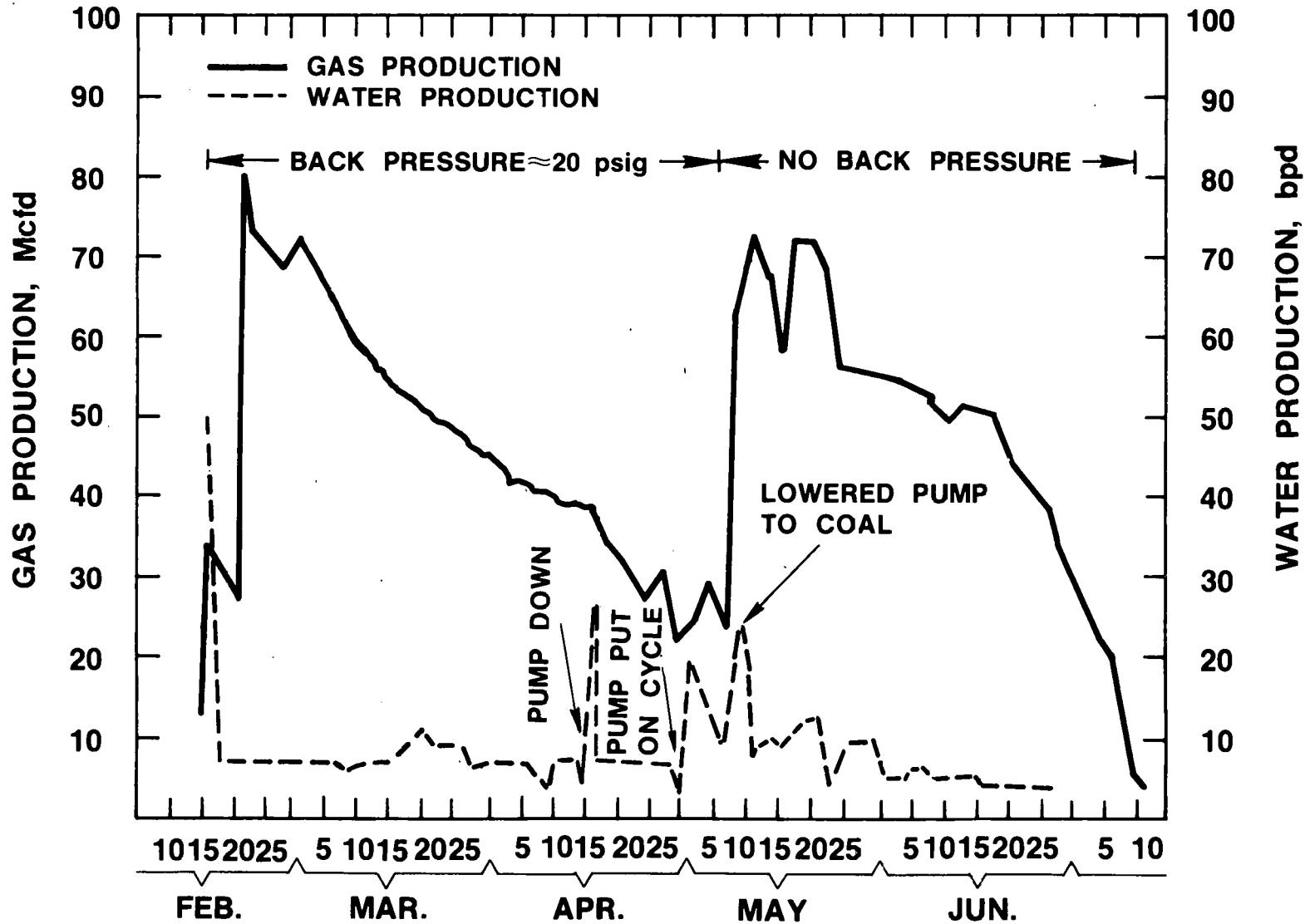
FIGURE 61. - DAILY PRODUCTION FROM TW5, MARY LEE COALBED, JEFFERSON COUNTY, ALABAMA.
