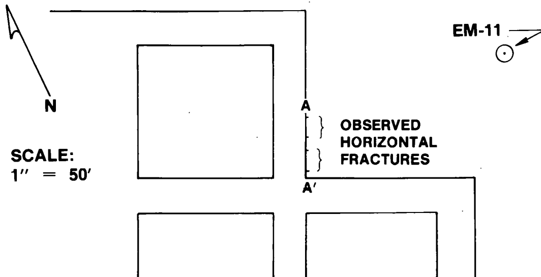
FIGURE 59. - SKETCH SHOWING POSITION OF THE INDUCED FRACTURES OBSERVED NEAR DEGAS WELL NO. EM-11 GREENE COUNTY, PA.
