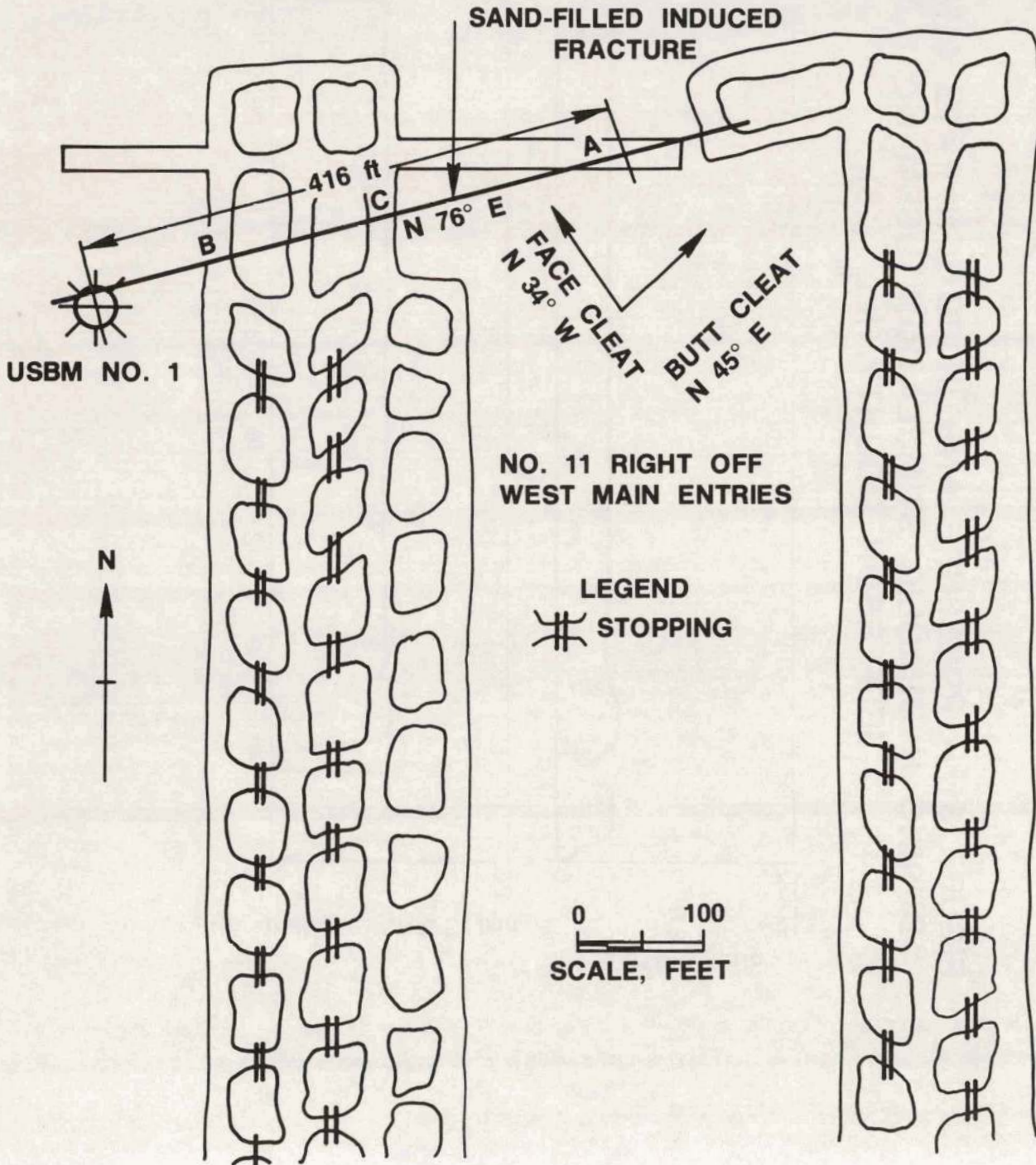
FIGURE 32. - INDUCED FRACTURE ORIENTATIONS AS RELATED TO MINE ENTRY DEVELOPMENT AT USBM NO. 1 NE, JEFFERSON COUNTY, ILL. (16).
