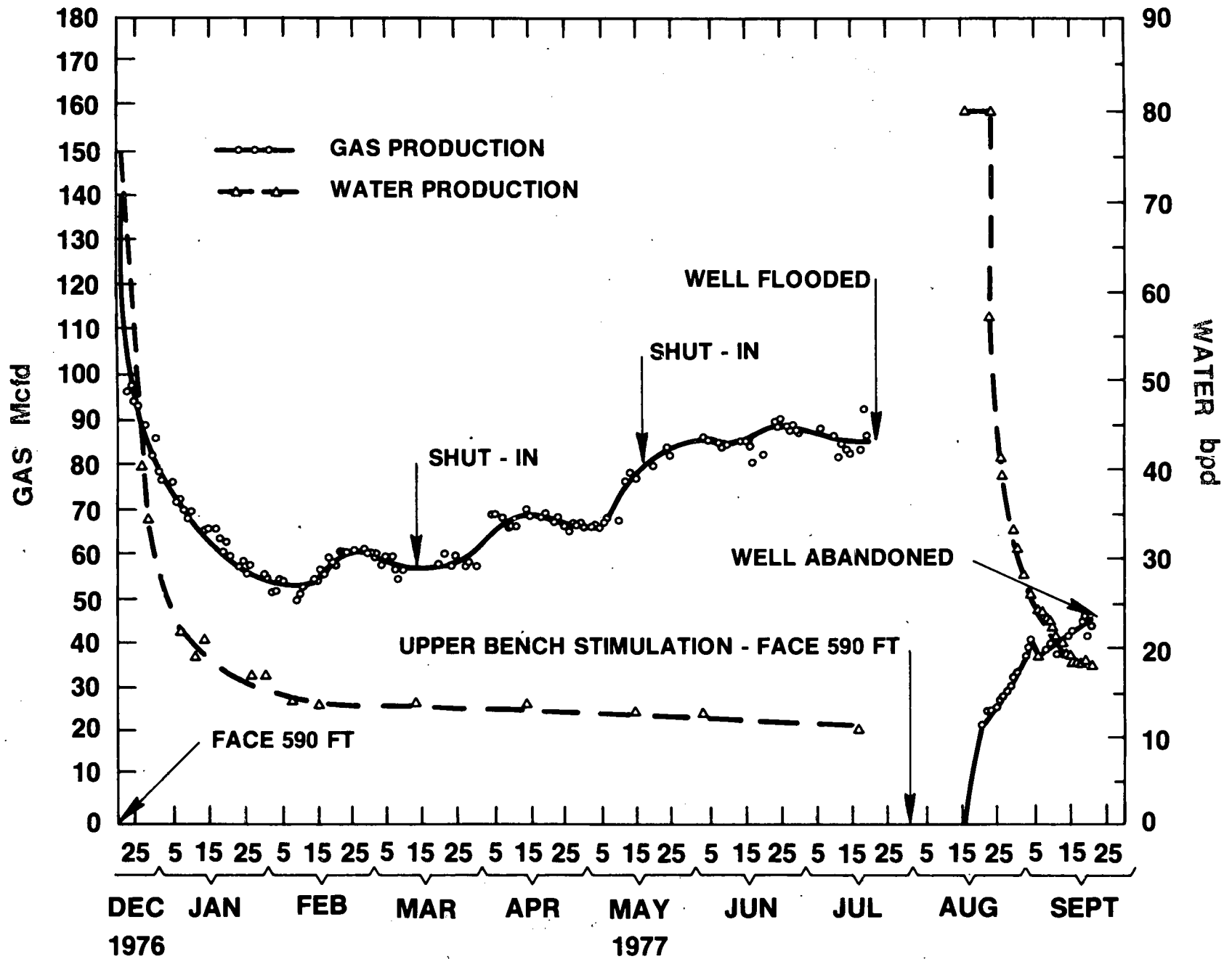
FIGURE 42. - PRODUCTION CURVES FOR TW3 (26).
