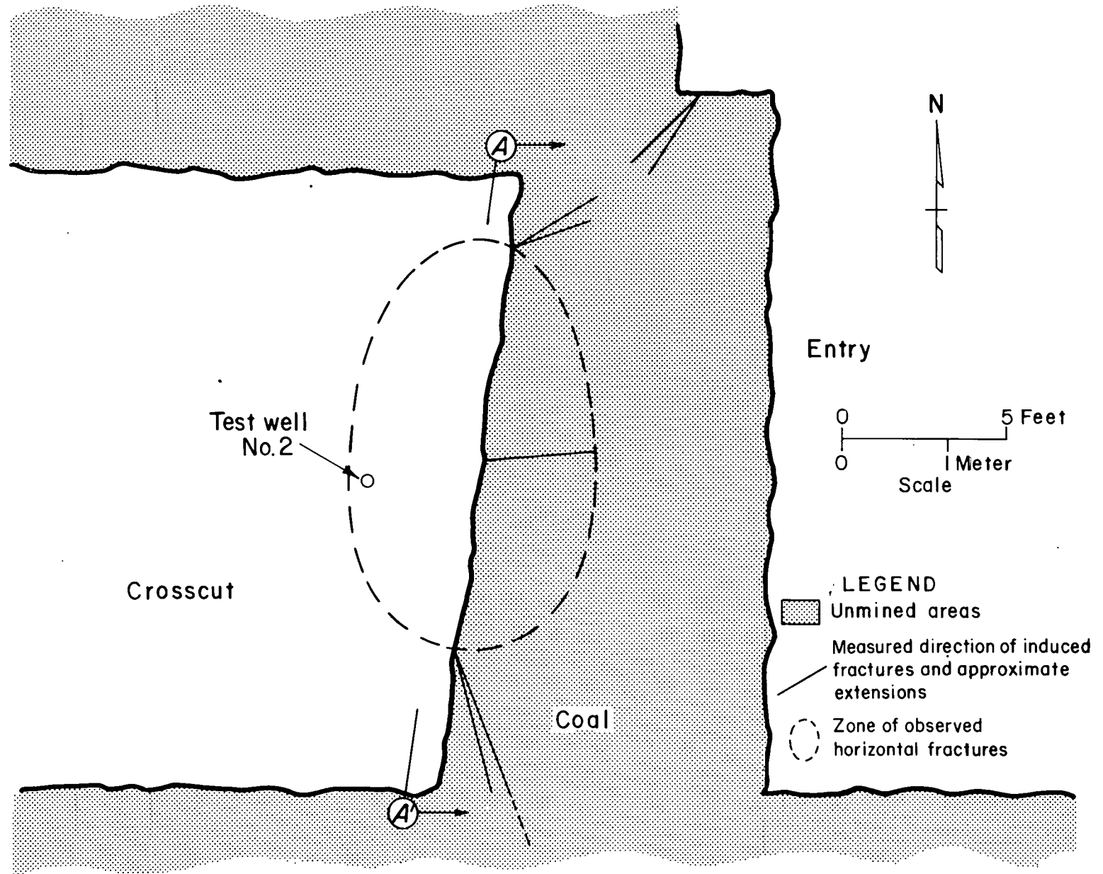
FIGURE 26. - POSITION OF MINE FACE DURING UNDERGROUND INVESTIGATION OF TW2 (23).
