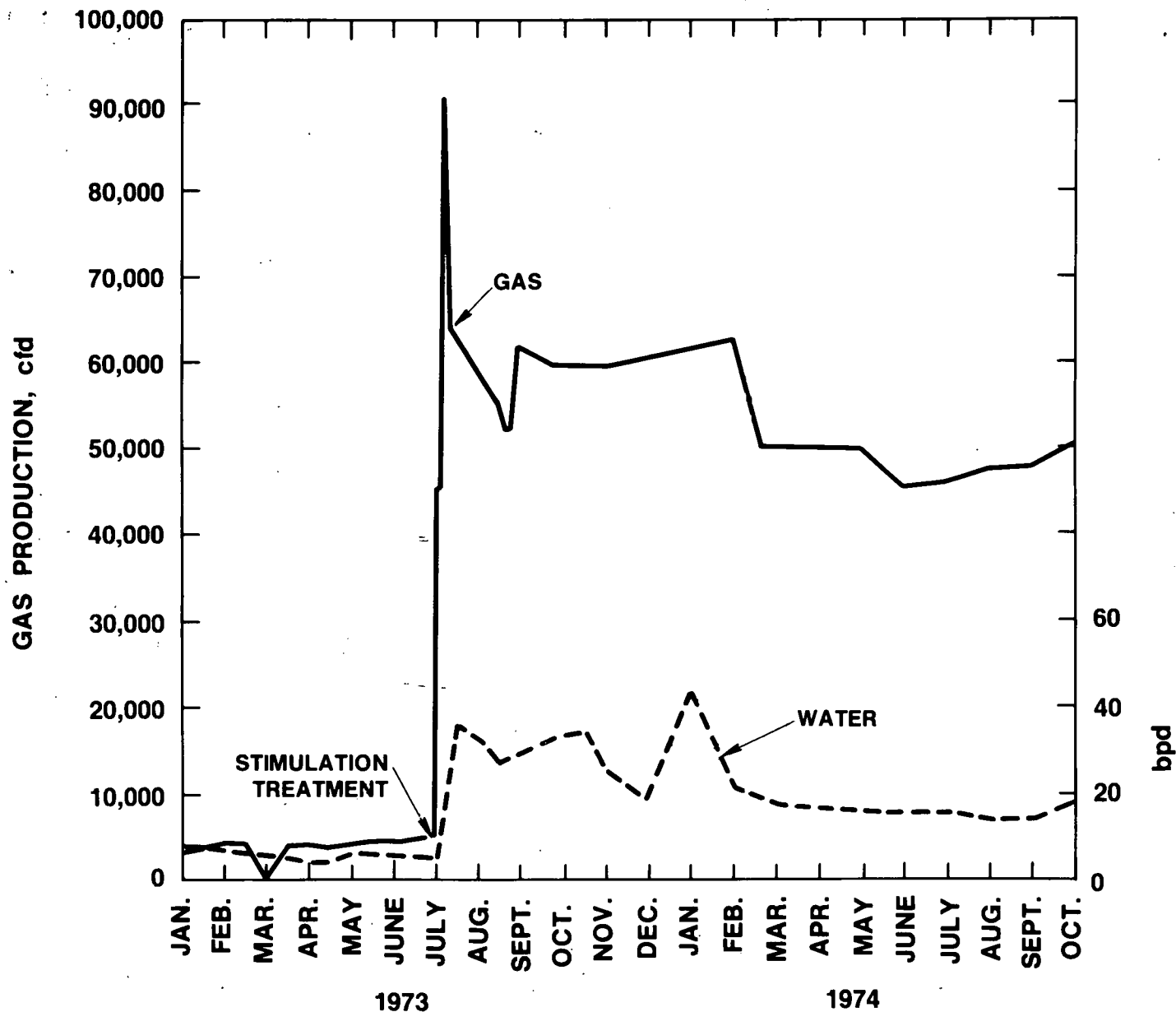
FIGURE 21. - GAS AND WATER PRODUCTION RATES BEFORE AND AFTER HYDRAULIC STIMULATION TREATMENT OF THE MARY LEE COALBED (7).
