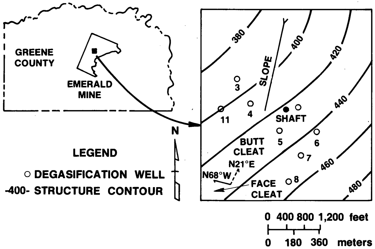
FIGURE 38. - PATTERN OF EIGHT DEGASIFICATION WELLS LOCATED ON EMERALD MINE PROPERTY, GREENE CO., PA. (37).
