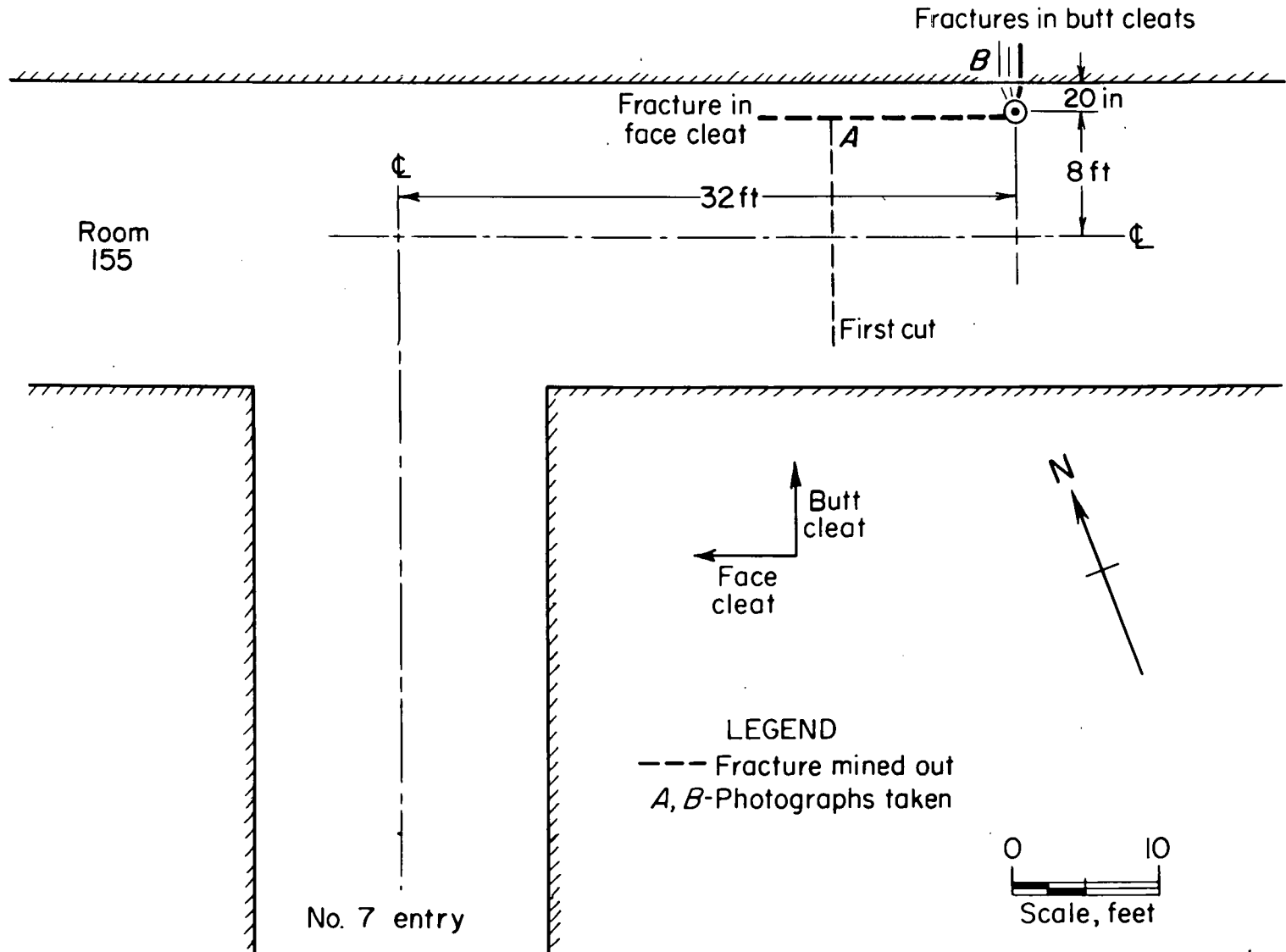
FIGURE 28. - INDUCED FRACTURE ORIENTATION RELATIVE TO MINE ENTRY DEVELOPMENT (16).
