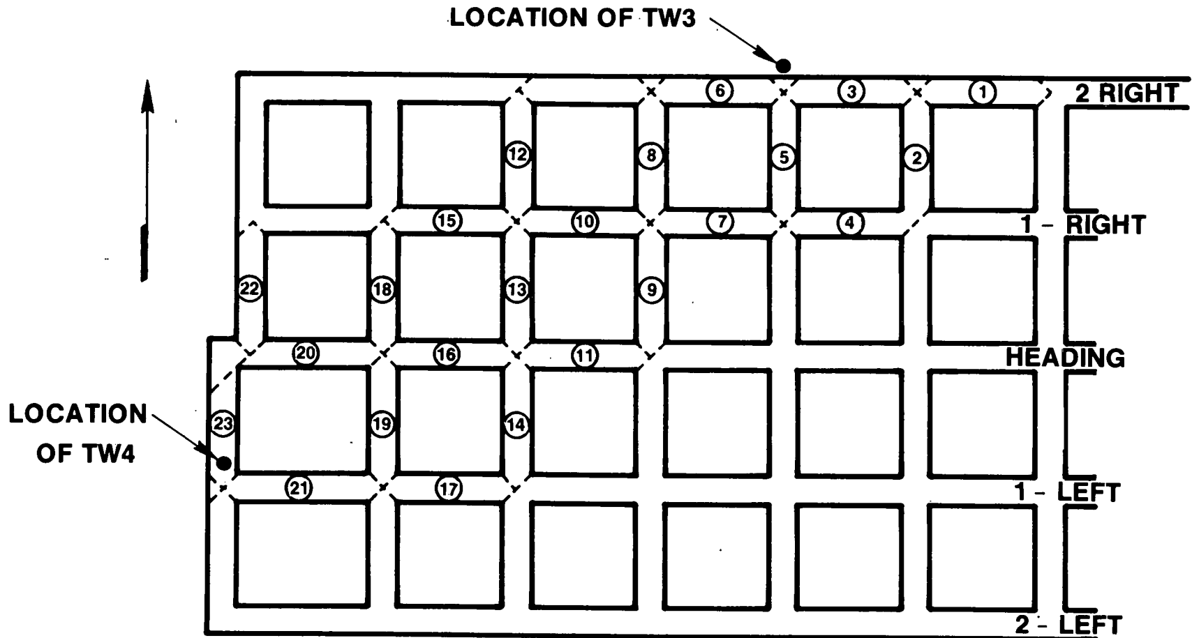
FIGURE 44. - SURVEY STATIONS DIVIDING AREA OF MINE NEAR TW3 AND TW4 (26).
