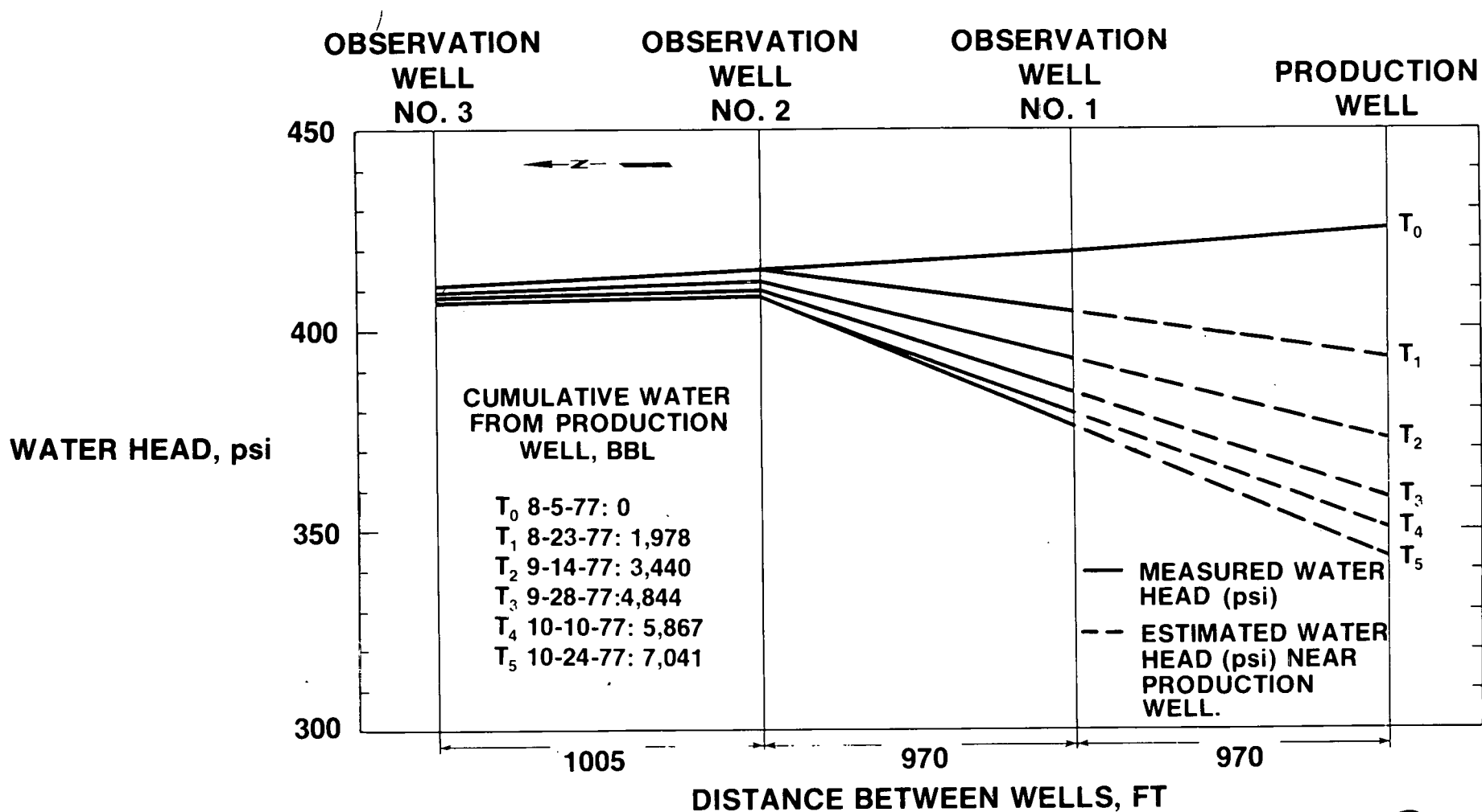
FIGURE 5. - COALBED WATER PRESSURE DECLINE MEASURED AT OBSERVATION WELLS PLACED ALONG A NORTH-SOUTH LINE AND UP TO 2,945 FEET FROM PRODUCTION WELL.
