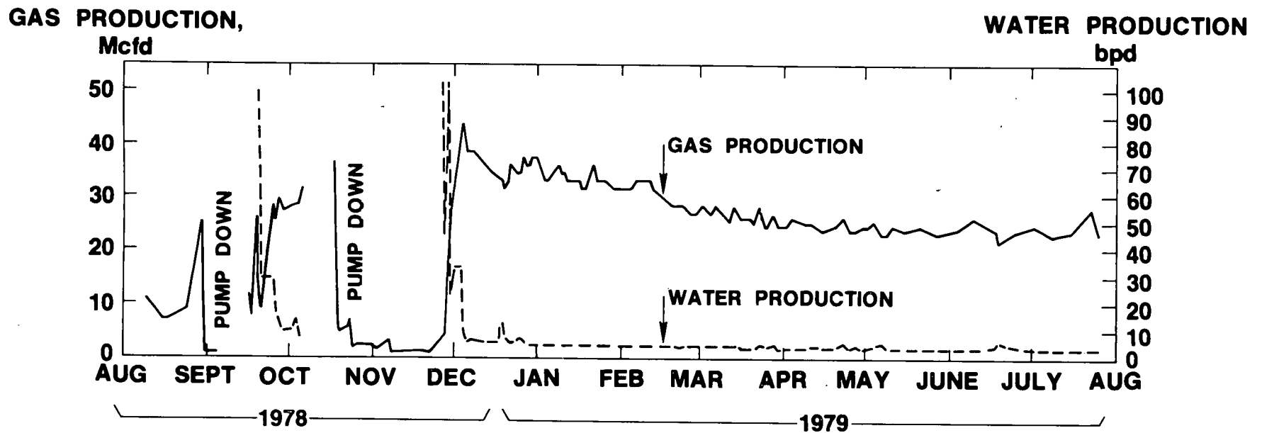
FIGURE 57 - DAILY GAS AND WATER PRODUCTION FROM WELL NO. DG-1A, DICKENSON COUNTY, VIRGINIA
