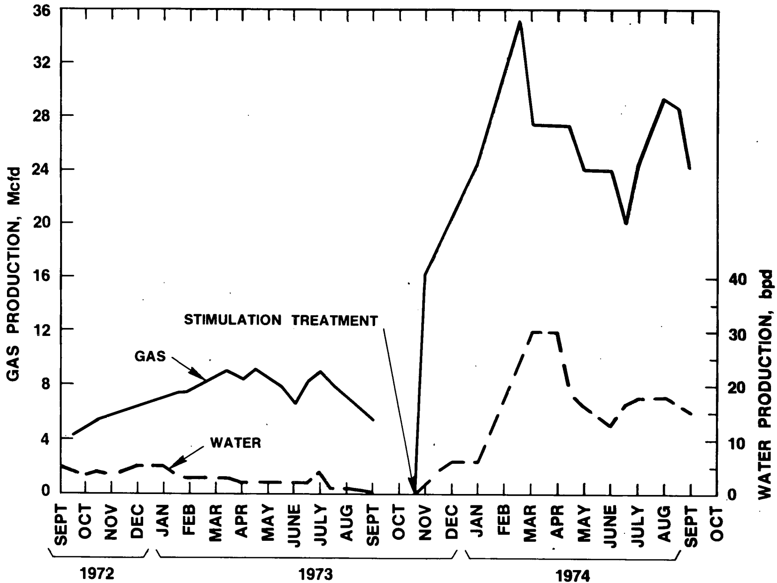
FIGURE 23. - GAS AND WATER PRODUCTION RATES BEFORE AND AFTER HYDRAULIC STIMULATION TREATMENT OF PITTSBURGH COALBED (14).
