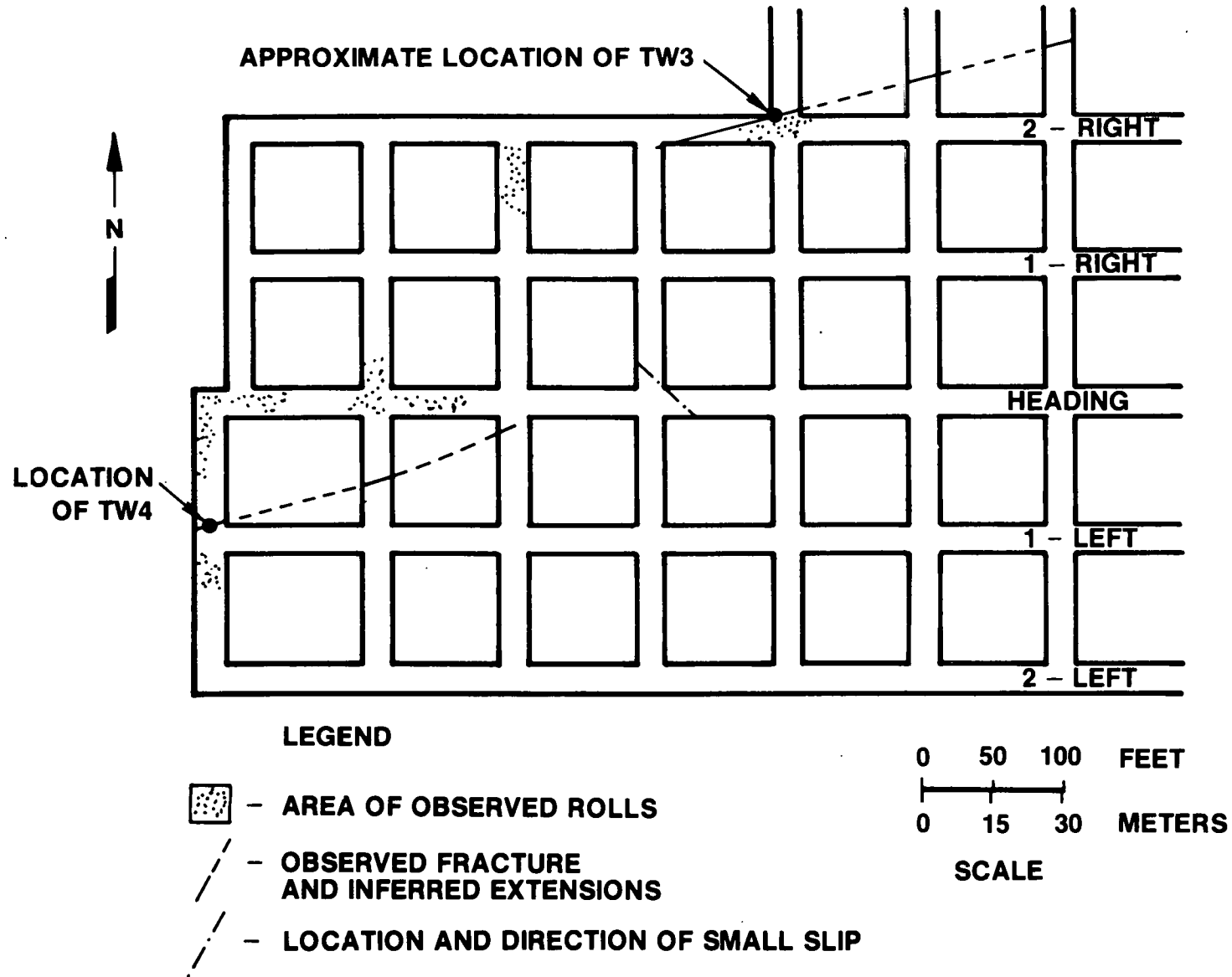
FIGURE 46. - PLAN VIEW OF MINE SHOWING TW3 AND TW4 LOCATIONS, TRACEABLE INDUCED FRACTURES AND OTHER FEATURES AS OBSERVED UNDERGROUND (26).
