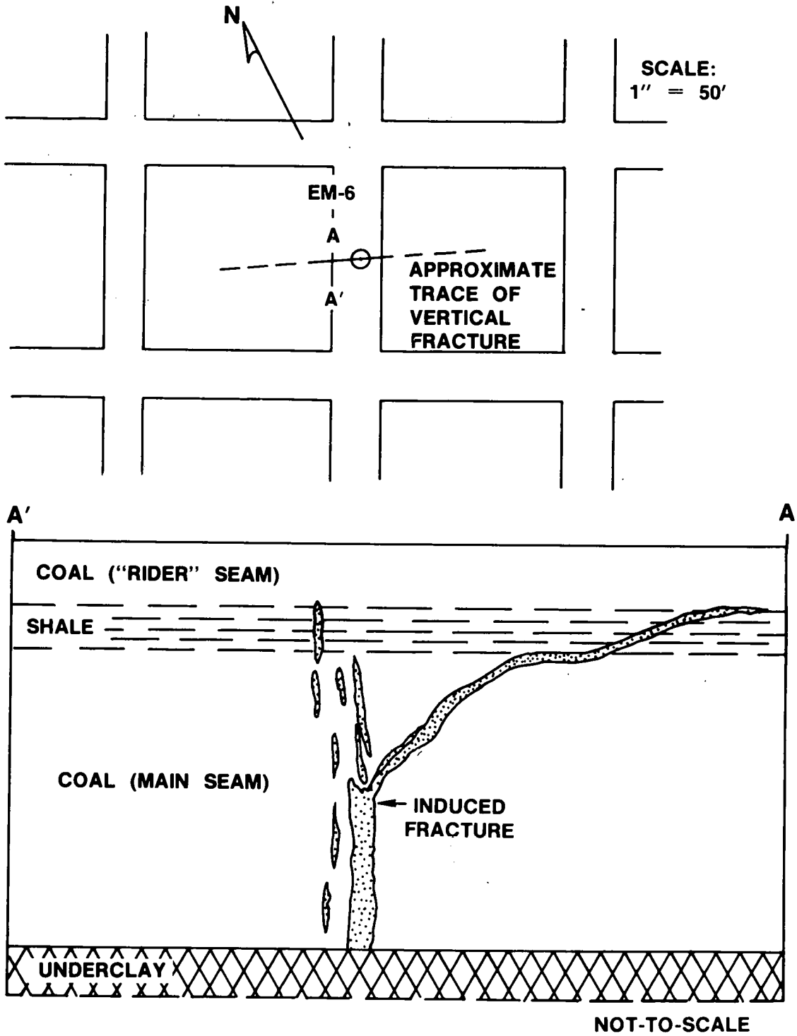
FIGURE 40. - POSITION AND ORIENTATION OF THE INDUCED FRACTURES OBSERVED NEAR DEGAS WELL NO. EM-6.
