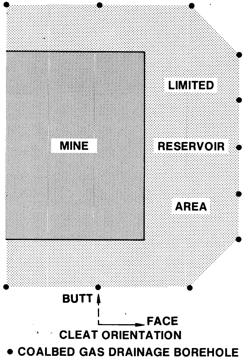
FIGURE 9. BOREHOLE ARRANGEMENT NEAR MINE WORKINGS.
