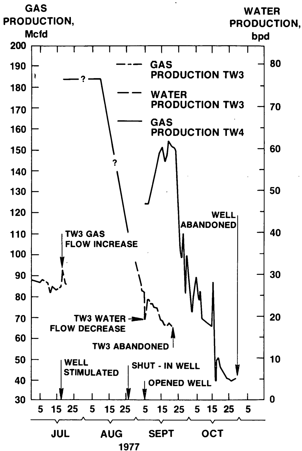
FIGURE 43. - PRODUCTION CURVES FOR TW4 AND PORTIONS OF TW3 (26).
