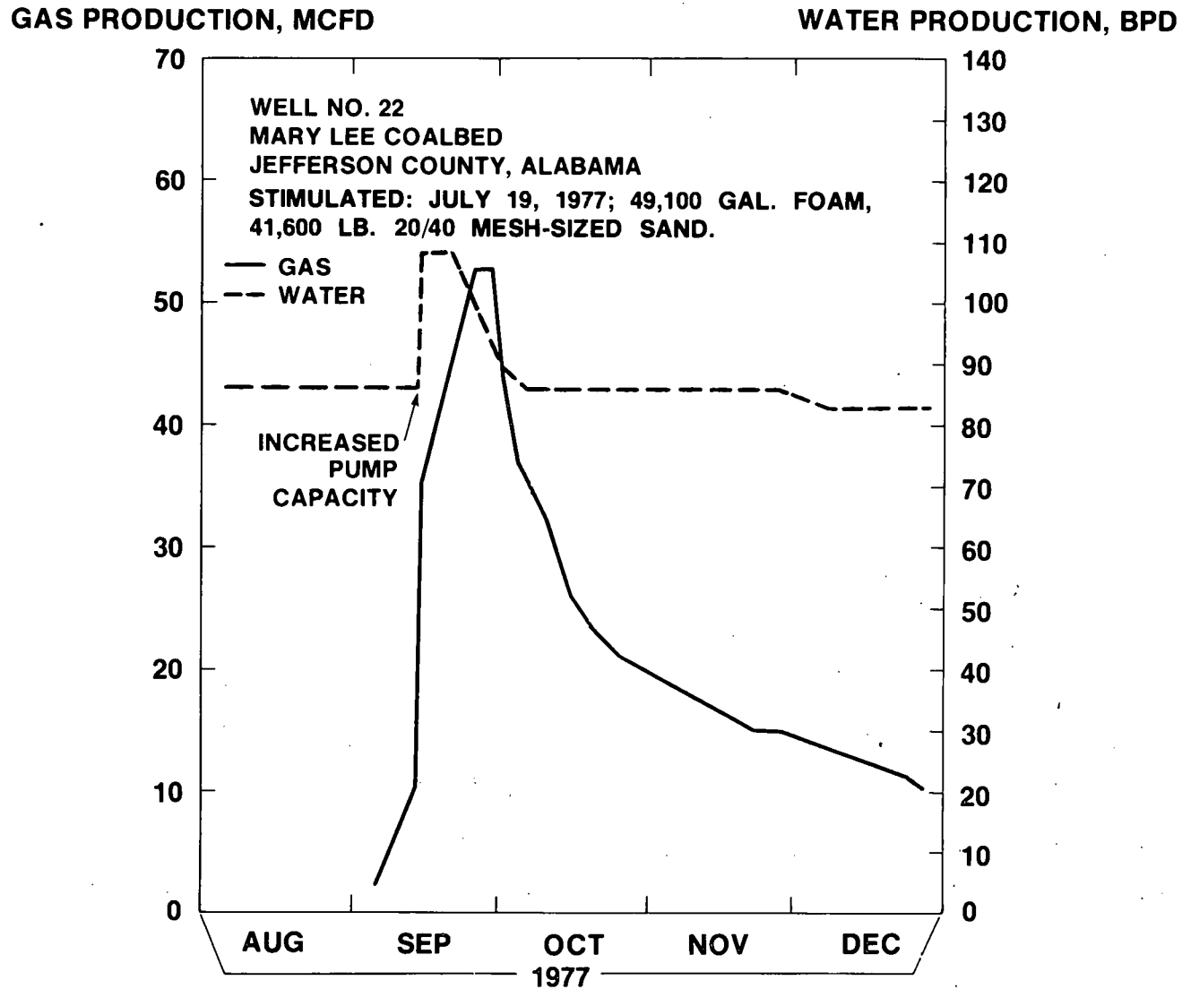
FIGURE 4. - PRODUCTION CURVES FROM A DRAINAGE WELL PLACED MORE THAN 3000 FEET FROM ANOTHER DRAINAGE POINT IN THE MARY LEE COALBED.
