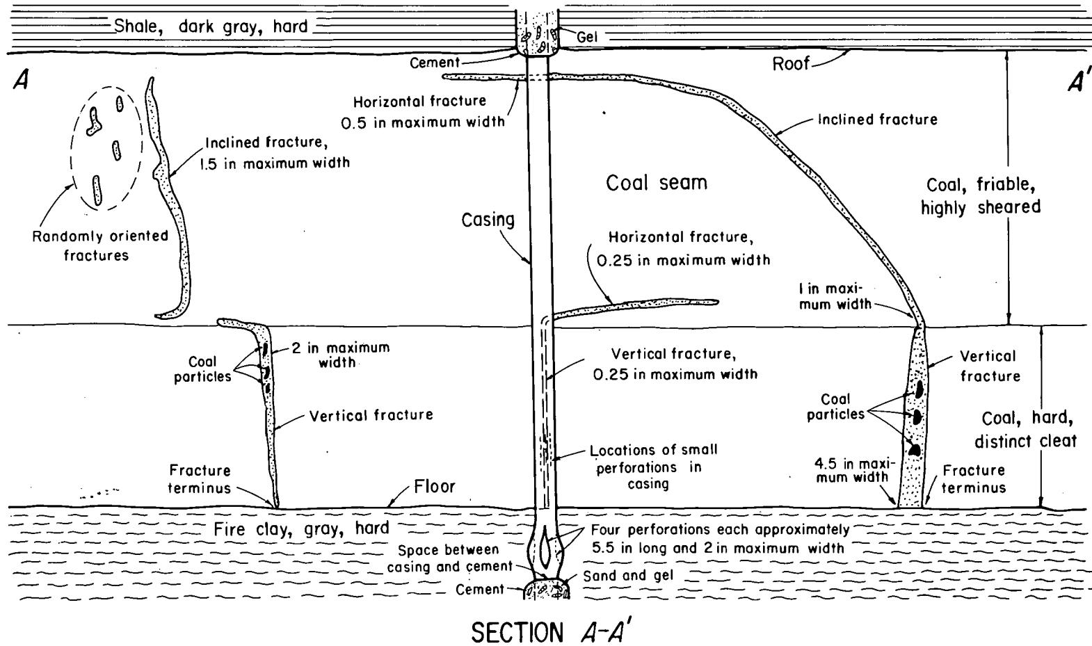
FIGURE 27. - SKETCH OF MINE FACE DURING UNDERGROUND EXAMINATION OF TW2 (23).
