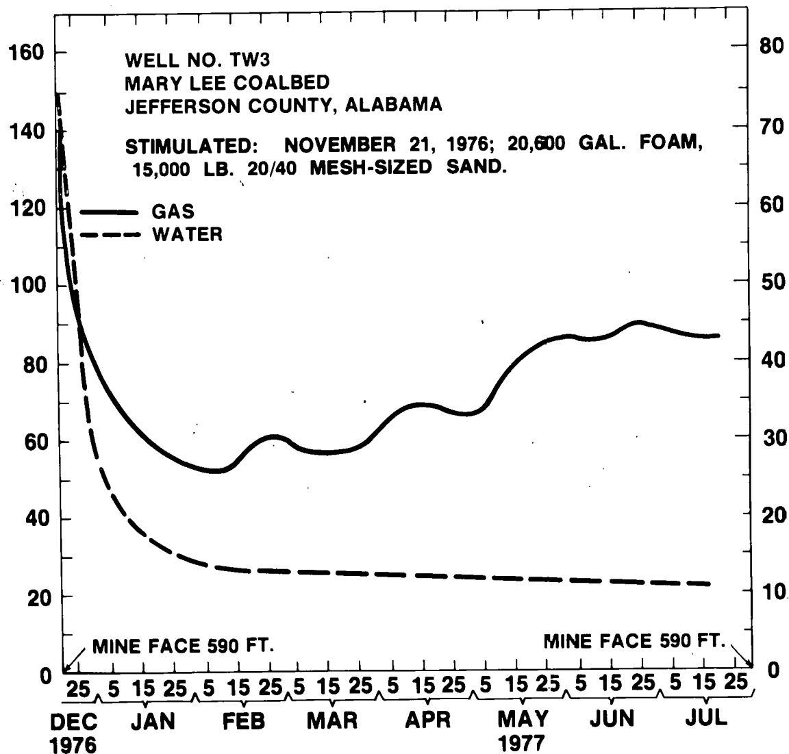
FIGURE 10. - PRODUCTION CURVES FROM A COALBED GAS DRAINAGE WELL PLACED NEAR MINE WORKINGS IN THE MARY LEE COALBED.
