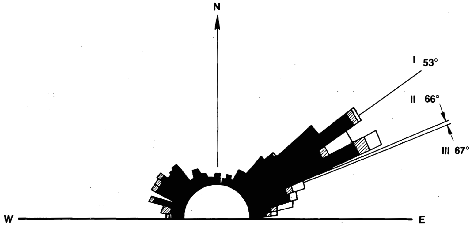
FIGURE 45. - COMPOSITE ROSE DIAGRAM OF TW3 AND TW4 SURVEY AREA SHOWING CLEAT, ROOF JOINT, AND INDUCED FRACTURE DIRECTIONS.
