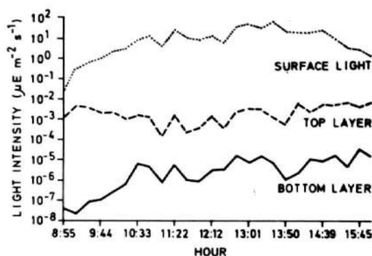
Fig. 7. Light intensities at surface and in centre of SSLs 8 January 1989, calculated from distribution of SSLs (Fig. 6).
