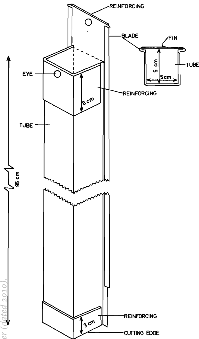
Fig. 1 Diagram of the corer showing the interlocking blade.
