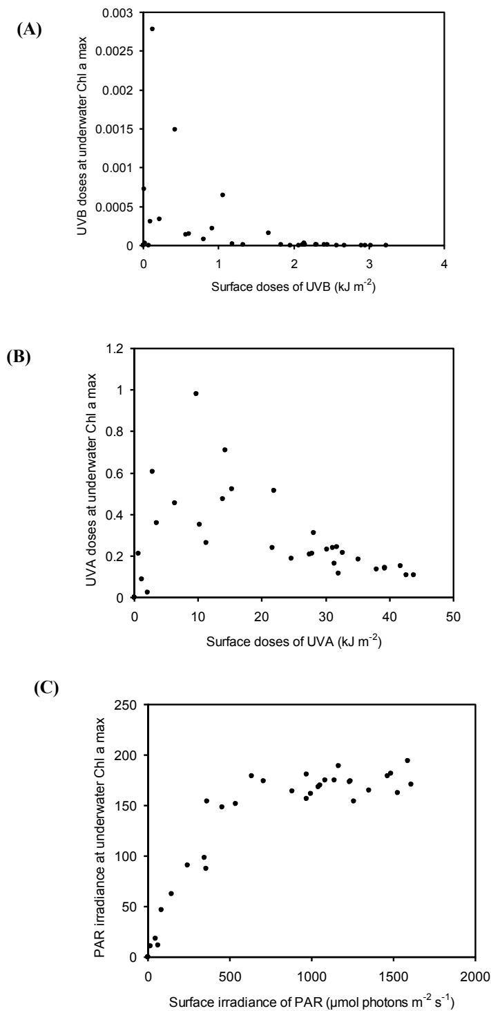
Figure 5 Surface irradiances/doses versus underwater irradiances/doses. Surface versus underwater irradiances/doses at the chlorophyll a maximum depth (Chl a max.) at Helgoland for the different wavelength ranges UVB (A), UVA (B) and PAR (C) including all data from profiles with pronounced chlorophyll a maxima. Values at both axes are in the energetic unit kilojoules per metre squared for UVB (A) and UVA (B) and in the quantametric unit micromoles of photons per meter squared per second for PAR (C); calculations see M&M.
