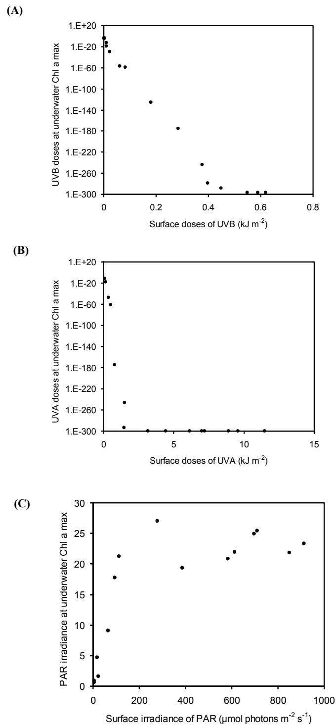
Figure 6 Surface irradiances/doses versus underwater irradiances/doses. Surface versus irradiances/doses at the chlorophyll a maximum depth (Chl a max.) at Hiddensee for the different wavelength ranges UVB (A), UVA (B) and PAR (C) including all data from profiles with pronounced chlorophyll a maxima. Values at both axes are in the energetic unit kilojoules per metre squared for UVB (A) and UVA (B) and in the quantametric unit micromoles of photons per meter squared per second for PAR (C); calculations see M&M.
