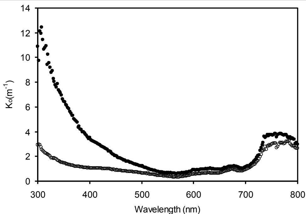
Figure 2 Attenuation spectra ( K_0 = overall attenuation coefficient). Attenuation spectra within water bodies of Helgoland (open circles) and Hiddensee (filled circles) calculated from five successive scans measured at intervals of 5 to 50 cm.
