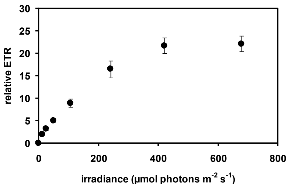
Figure 7 The rETR of phytoplankton. rETR of phytoplankton is plotted versus irradiance ( n = 3 of the first 3 days of the spring campaign) determined in situ before sunrise (completed before 5:15 a.m.) at study site Helgoland. The light saturation of photosynthesis ( E_k , quotient of P_{max} and alpha) was calculated to be around 219 \mu\text{mol photons m}^{-2} \text{s}^{-1} .
