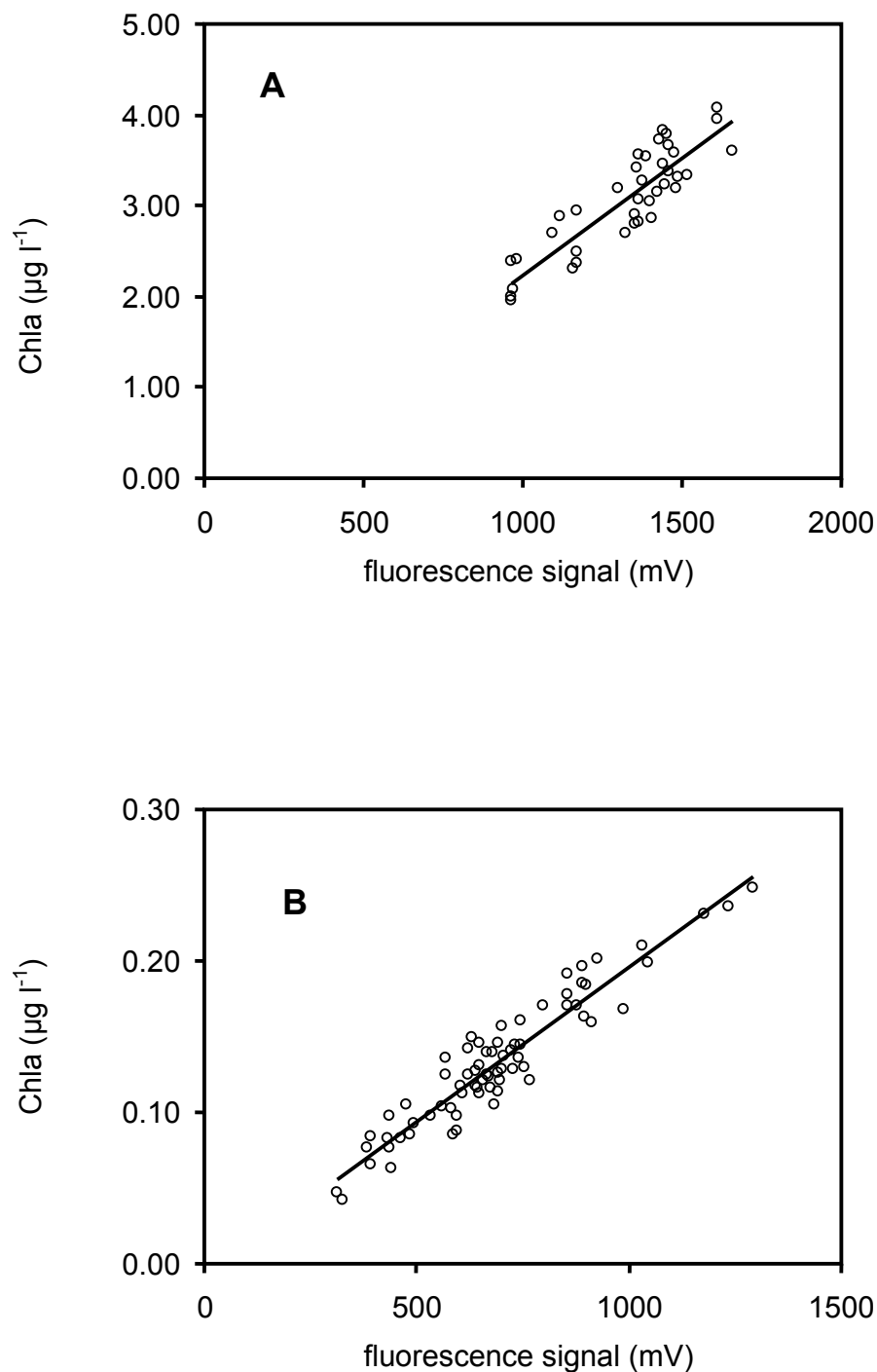
Figure 1 Calibration of the in vivo chlorophyll fluorometer, Fluorescence signals (millivolts) plotted versus the chlorophyll a concentrations (Chl a ), determined in situ and in water samples, respectively, within corresponding water depths at Hiddensee (A) and Helgoland (B). All data of vertical, spatial and temporal variations determined over the whole field campaigns are included.
