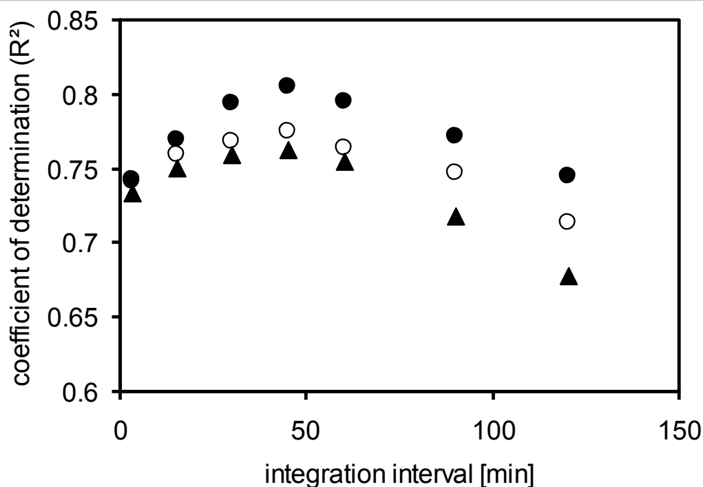
Figure 4 Coefficient of determination ( R^2 ) values of the linear regression. Shown are determination coefficient values between sub-surface irradiances/doses, calculated for different integration intervals, and chlorophyll a maximum depths. The different wavelength ranges of the sub-surface irradiances/doses are represented by filled circles (PAR 400 to 700 nm), open circles (UVA 320 to 400 nm) and triangles (UVB 290 to 320 nm).
