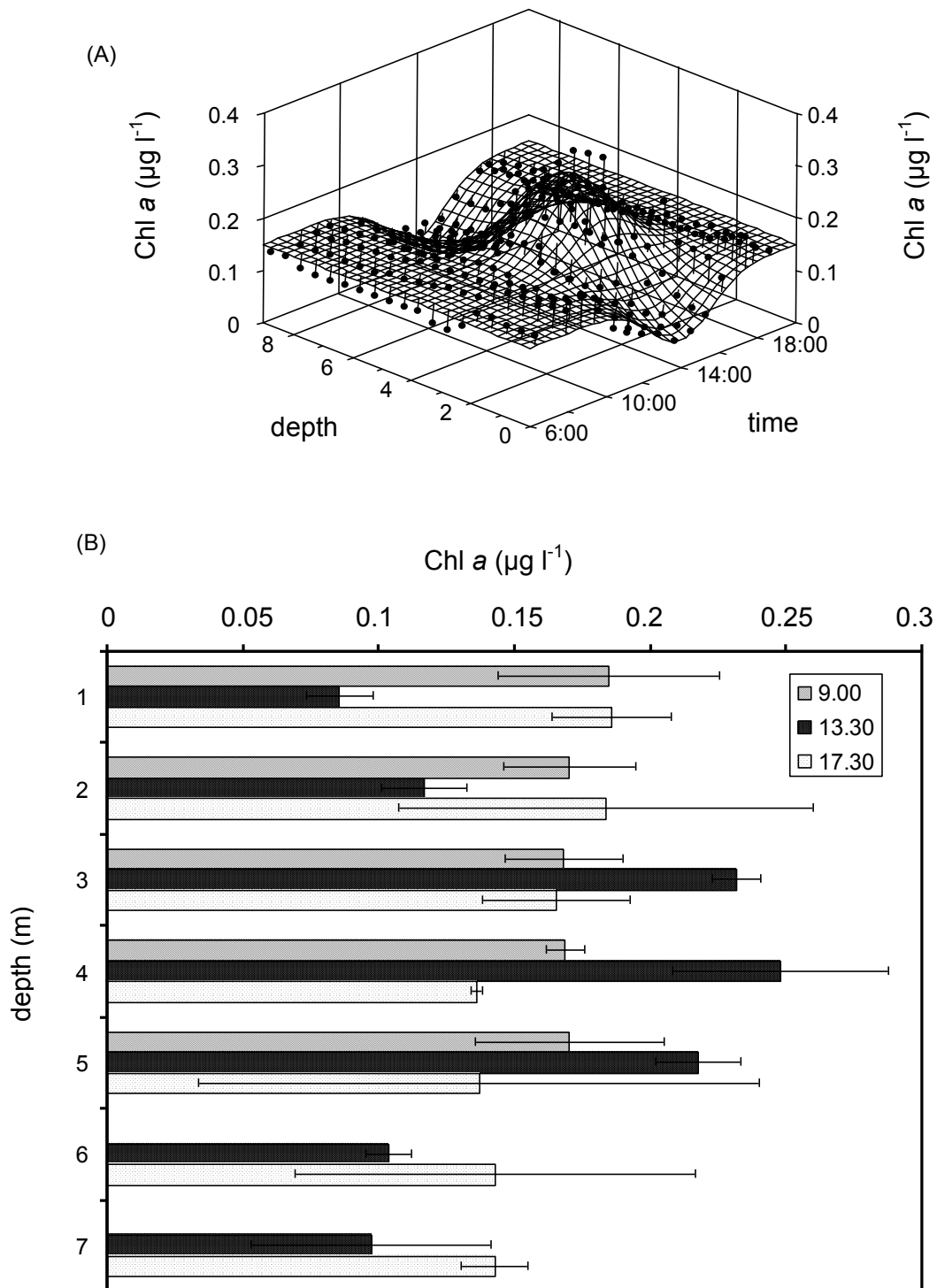
Figure 3 Vertical distribution of chlorophyll a concentration in the water column at study site Helgoland. Shown are vertical chlorophyll a profiles during the second day of the spring campaign. (A) shows a surface grid calculated from fluorescence data by means of a Gaussian fit procedure using TC3D software (see M&M). (B) shows Chl a concentration profiles determined by means of the DMF-extraction method taken the same day. Vertical bars denote standard deviation.
