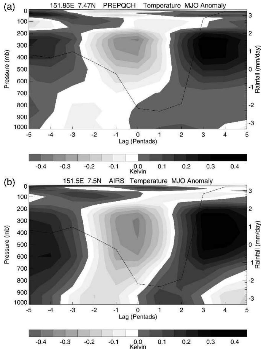
FIG. 15. MJO vertical temperature structure using (top) radiosonde and (bottom) AIRS at Truk ( 7.47^{\circ}\text{N} , 151.85^{\circ}\text{E} ). The superimposed solid black line denotes the collocated TRMM rainfall anomaly ( \text{mm day}^{-1} ).
