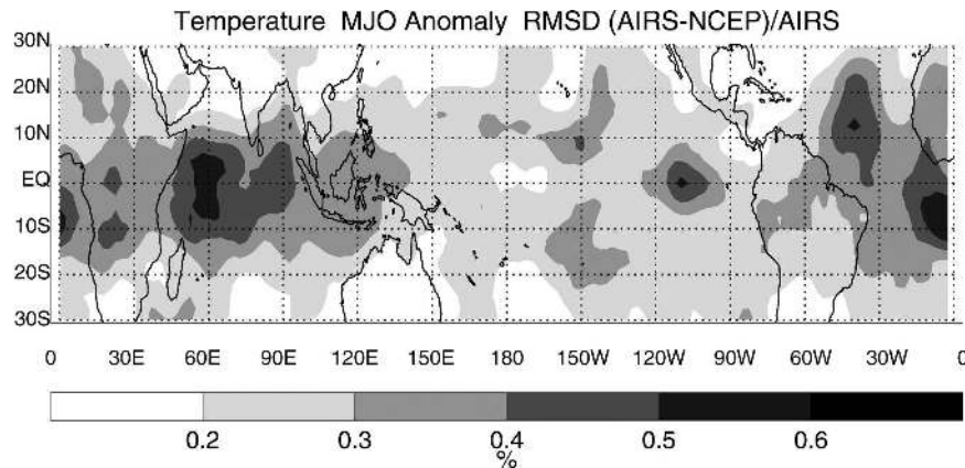
FIG. 14. Temperature anomaly root-mean-square difference (RMSD) between AIRS and NCEP.
