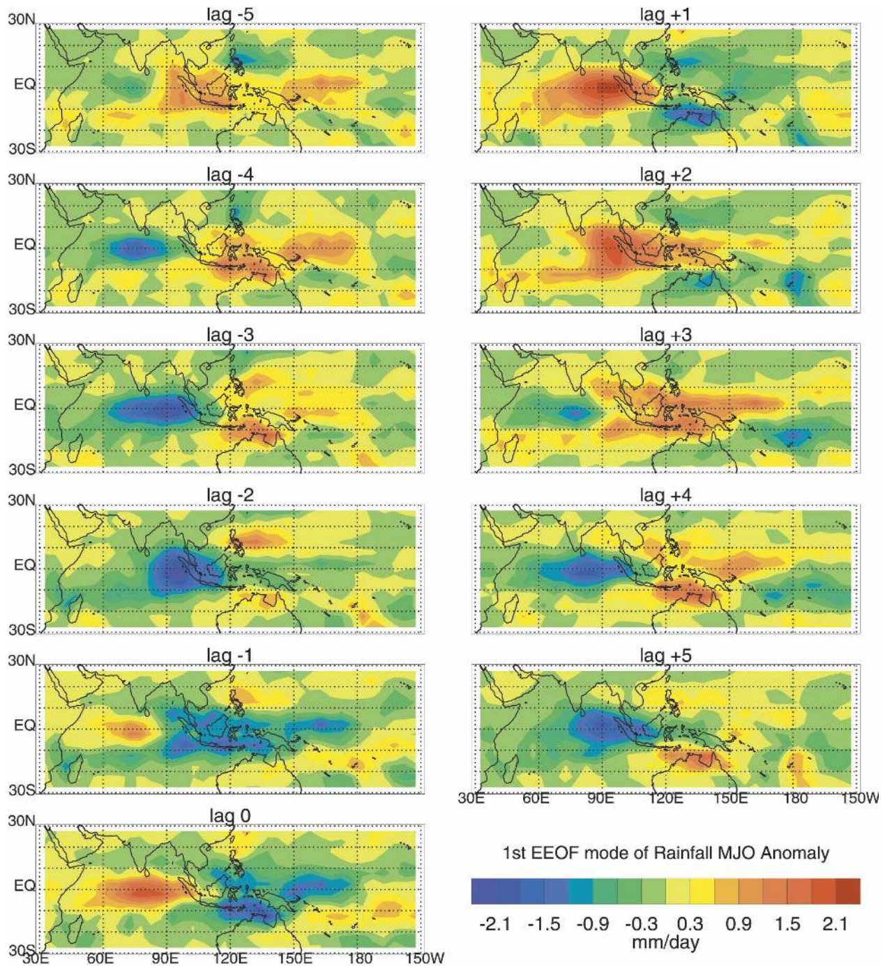
FIG. 1. Spatial-temporal pattern for the first EEOF mode of TRMM rainfall anomaly from NH wintertime (November–April) and the region 30°N–30°S and 30°E–150°W. The unit for the lag is pentad. The color red denotes positive rainfall anomalies, i.e., enhanced convection, while the color blue indicates negative rainfall anomalies, i.e., suppressed convection.
