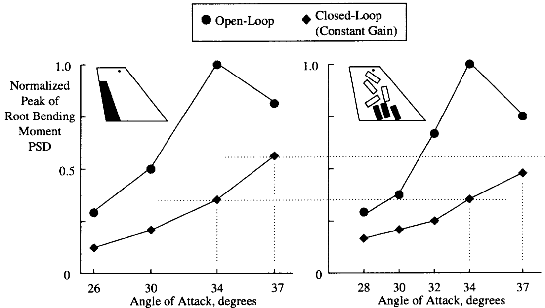
(a) Rudder Results (b) Piezoelectric Actuator Results Figure 17. Comparisons of the Peak Values of the PSD of the Root Bending Moment at the Frequency of the First Bending Mode for Open-Loop and Closed-Loop Conditions, At Various Angles of Attack, 14 psf
