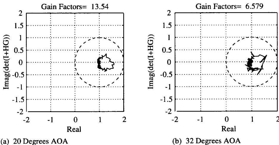
(a) 20 Degrees AOA (b) 32 Degrees AOA Figure 18. Expected Performance of the Baseline Control Law For 2 Angles of Attack, 14 psf
