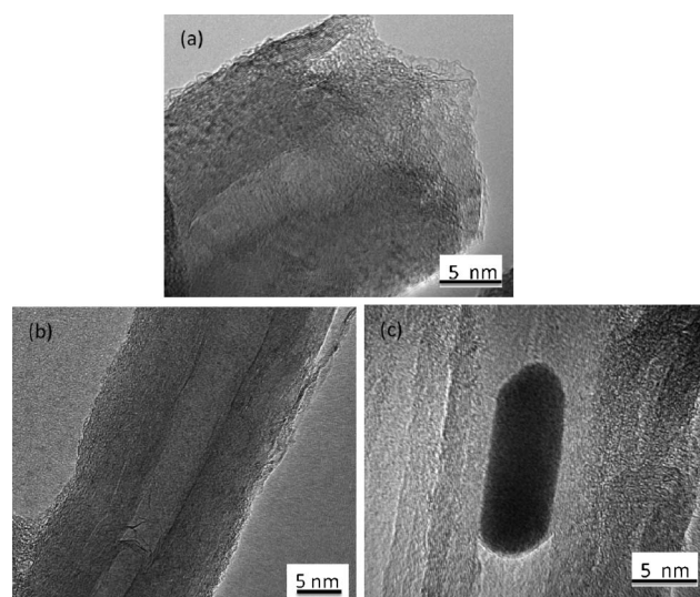
Fig. 5 (a) Typical HRTEM image for the tip removed CNT by mechanical sanding (b) Bamboo structure CNT (c) iron catalyst migrated into the channel.
