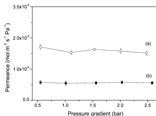
Fig. 6 Argon permeances through vertically aligned carbon nanotube membranes at 20 °C (a. VACNT-M1, b. VACNT-M2).
