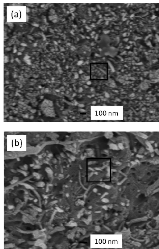
Fig. 4 SEM images of top surface of CNT membranes after mechanical polishing (a: VACNT-M1, b: VACNT-M2).
