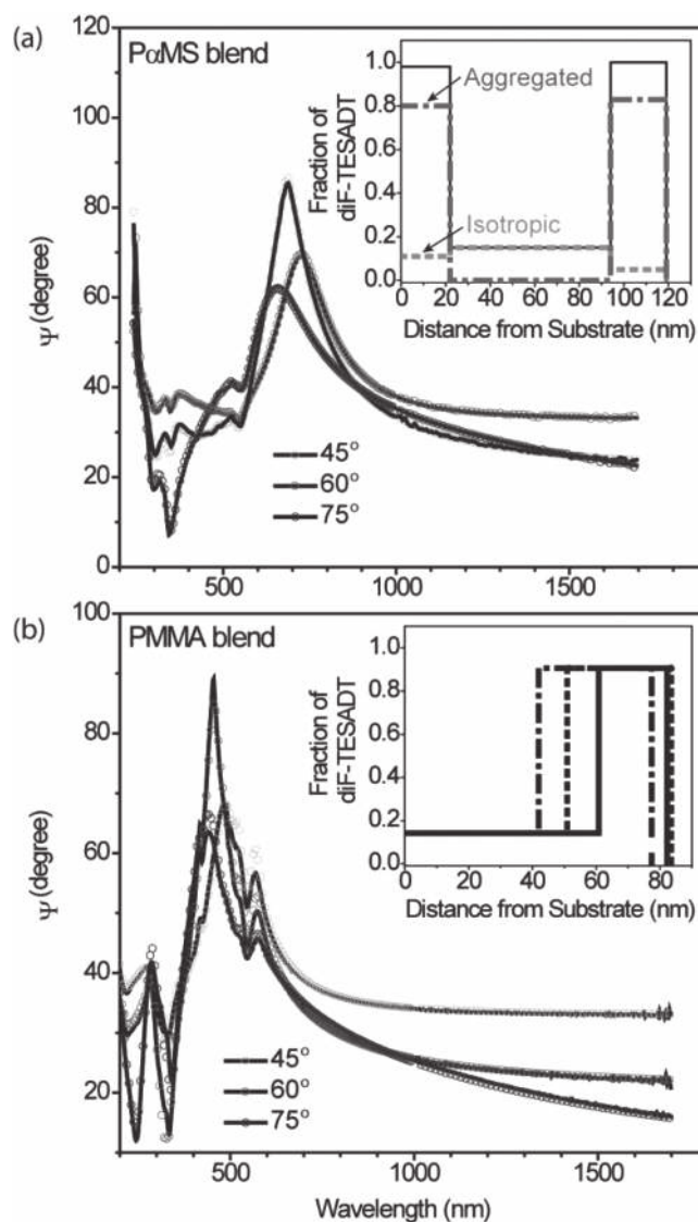
Figure 4. a) Spectroscopy ellipsometry angle \Psi for three angles of incidence (solid line) and model fit (open circle) for data from a P \alpha MS blend film on a native oxide substrate. Inset shows the derived depth profile for diF-TESADT volume fraction (solid line). Also shown is the amount of diF-TESADT in the isotropic dispersed state (gray short dash) and aggregated material with a (001) orientation (gray dash dot). b) \Psi for three angles of incidence (solid line) and model fit (open circle) for data from a PMMA blend film on a native oxide substrate. Inset shows the derived depth profile for diF-TESADT volume fraction from each of the three substrates modeled: native (solid line), thermal (short dash), and fused silica (dash dot).
