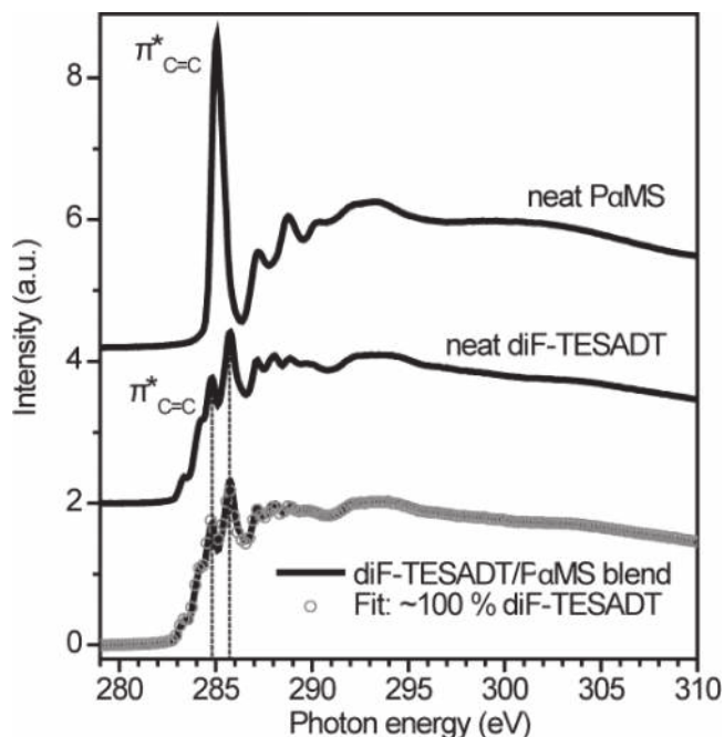
Figure 7. The carbon K-edge NEXAFS data of pure component films and a top film of diF-TESADT/P \alpha MS blend system. The composition of the top interface is found to be \approx 100\% diF-TESADT. Spectra are offset for clarity. Standard uncertainty in intensity (PEY) is \pm 2\% ; photon energy \pm 0.2 eV.
