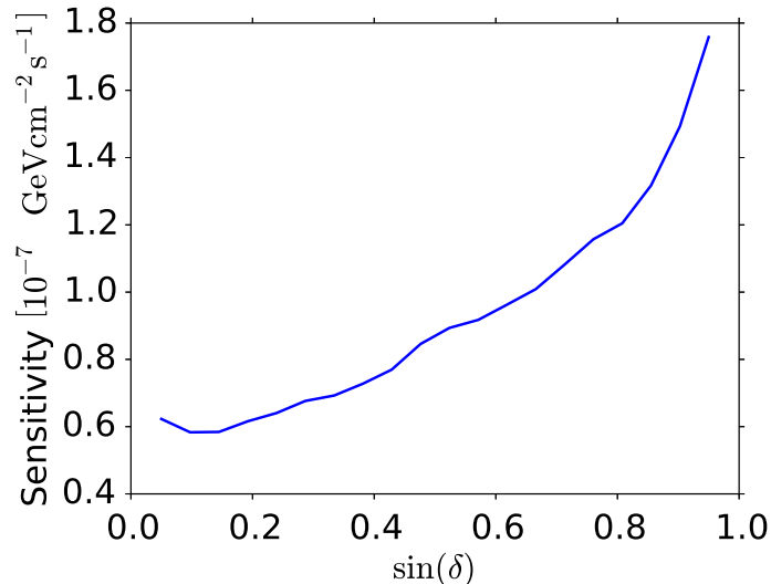
Figure 1. Simulated IceCube sensitivity as a function of source declination to a neutrino flux with dN/dE \sim E^{-2} for a neutrino flare length of 10 days and for the IC-2012 data set. The sensitivity did not change significantly for other IceCube data seasons. The sensitivity is defined as the flux required for a 3 sigma detection with a probability of 90%.
