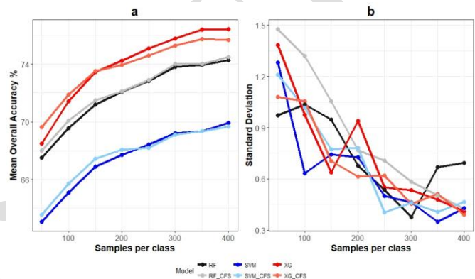
Fig. 3. Mean overall accuracy and standard deviation of 10 random distributions of training data for each sample size category
