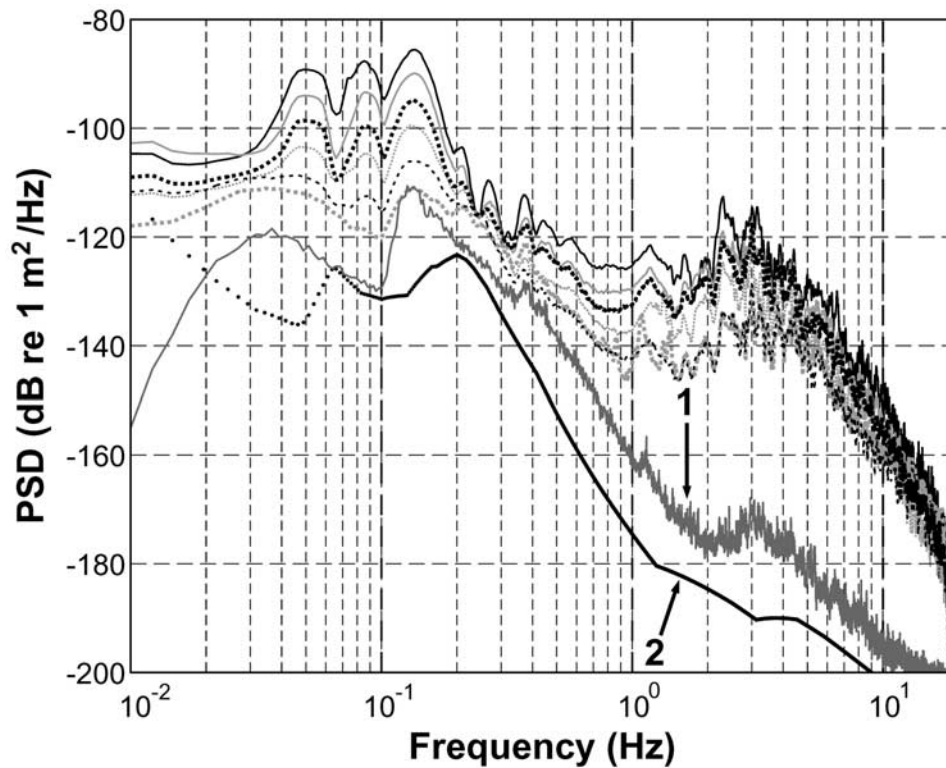
Figure 12. Displacement power spectral densities from 109 explosions recorded between 1 January and 24 April 2001 at EIS, stacked within six equal power bands. Also shown are average pre-event noise (1) and a global average noise model (2) spectrum from Peterson [1993]. Note the relative scaling of SP and VLP band spectral amplitudes, and nearly constant VLP and SP frequency peaks, over an \sim 20 -fold range of event sizes. VLP spectral changes for the smallest events are seen from the noise PSD (1) to be the result of background microseism noise. Noise falloff at periods greater than 30 s relative to the Peterson model is due to the 30-s seismometer low response corner. Spectra are estimated using 200-s multitapers [Thomson, 1982] with a spectral resolution of \pm 0.01 Hz.
