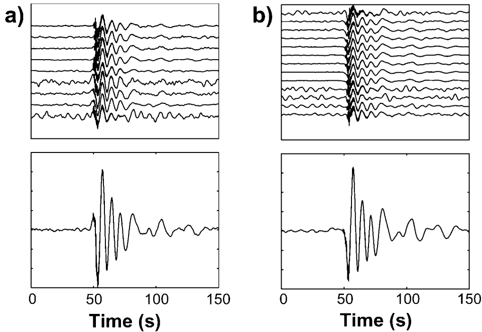
Figure 7. Representatives of VLP event families recorded during 2001 at EIS (with respective stacks shown at bottom), displaying variable pre-ruptive VLP signal polarities: (a) upward and (b) downward. In contrast, the minutes-long VLP coda is much more repeatable across all events (Figure 3).
