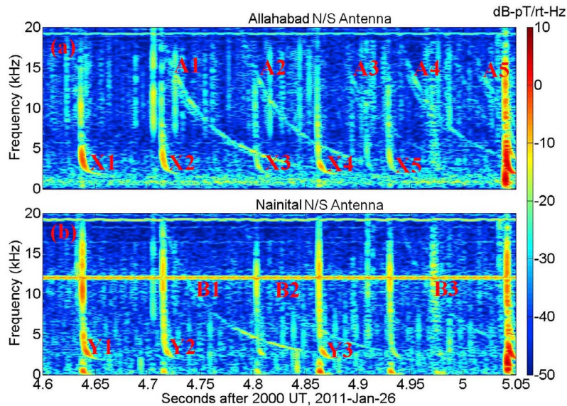
Figure 1. Spectrograms showing whistlers observed simultaneously at both stations (a) Allahabad and (b) Nainital on 26 January 2011 after 20:00:4.5 UT (01:30:4.5 LT). The color scale shows the intensity or amplitude of recorded signal.
