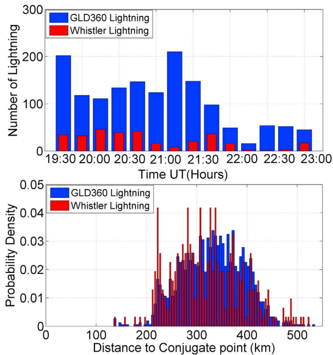
Figure 3. (top) The temporal evolution in the occurrence pattern of GLD360 detected lightning strikes (blue bars) and whistler producing lightnings (red bars) between 19:30–23:00 UT. (bottom) The distance to the conjugate point of the 1508 GLD360 lightning strikes (blue bars) and 311 whistler producing lightning strikes (red bars).
