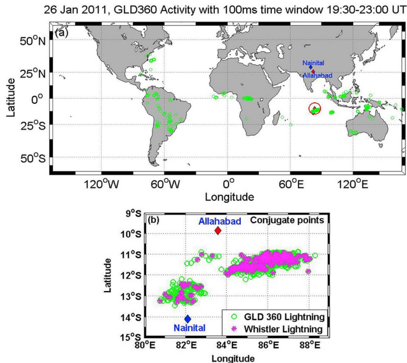
Figure 2. (a) Locations of receiving stations Allahabad and Nainital on global map along with GLD360 detected lightning locations with \leq 100 ms time window prior to occurrence time of each whistler during 19:30 UT to 23:00 UT (green circles). Red circle of 600 km radius shows a well confined zone of lightning activity surrounding the conjugate point. (b) Zoom in view of the conjugate area to show the conjugate points of receiving stations with respect to GLD 360 detected lightning strikes (green circles) and whistler producing lightning strikes (magenta colored stars).
