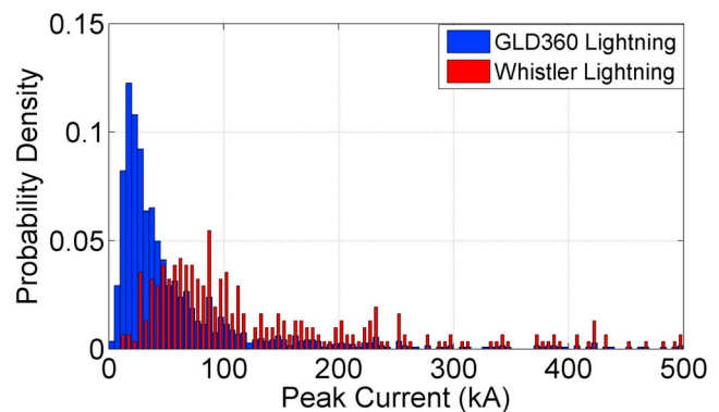
Figure 4. The probability distribution of peak currents (kA) of all GLD360 lightning strikes in the storm (blue bars) and whistler producing strikes (red bars).
