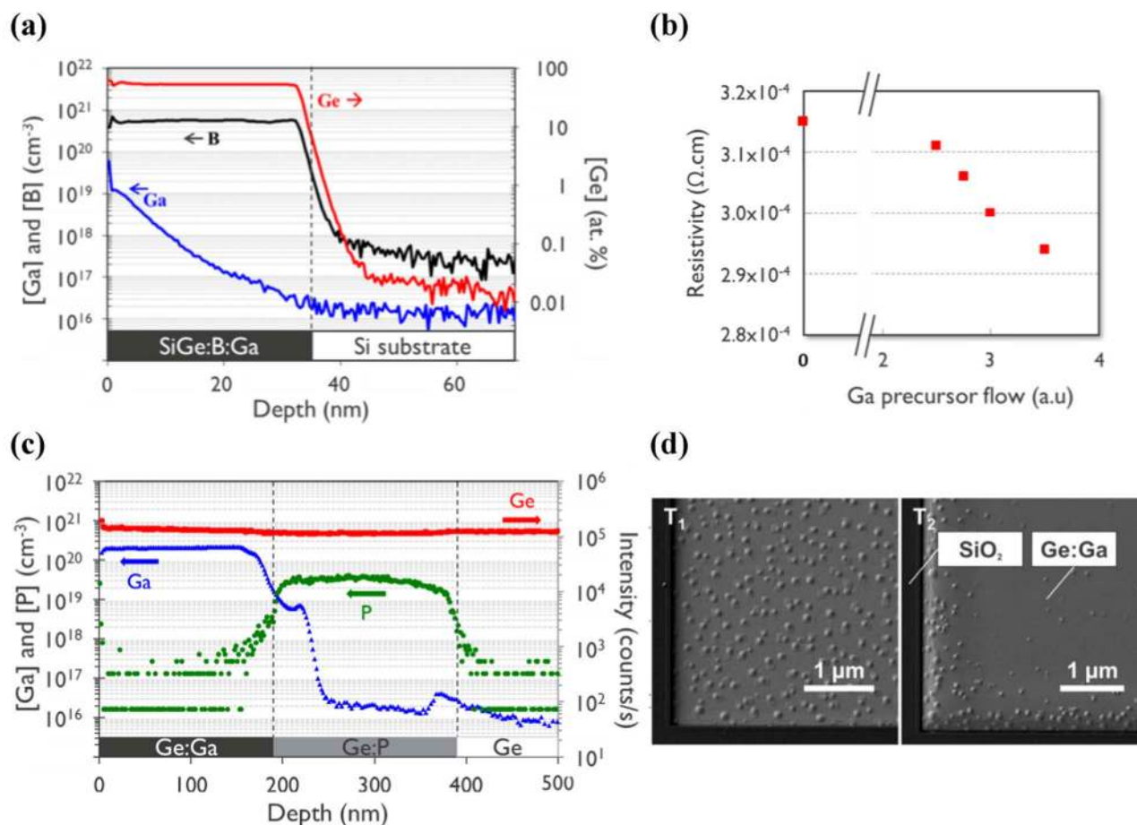
Figure 4. (a) B, Ga and Ge SIMS profiles extracted from a 35 nm thick Si 0.5 Ge 0.5 :B:Ga layer directly grown on Si. (b) SiGe:B:Ga resistivity as a function of Ga precursor flow (ASM data). (c) Ga, P and Ge SIMS profiles measured in a 180 nm thick Ga-doped Ge layer, epitaxially grown on 200 nm Ge:P on Ge/Si. (d) SEM images of selectively grown Ge:Ga layers at two different growth temperatures T 1 and T 2 , all other conditions being the same. At temperature T 2 < T 1 , Ga clustering is clearly reduced.
