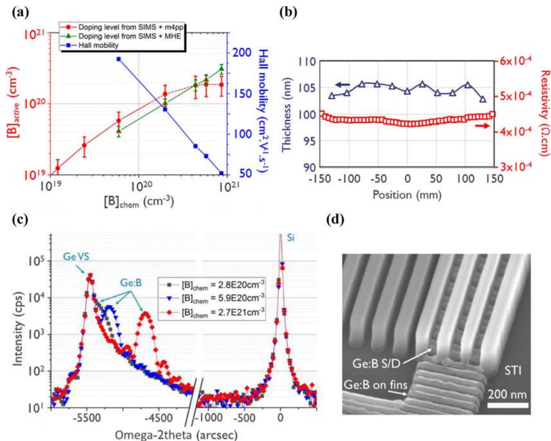
Figure 5. (a) Summary plot of SIMS, m4pp and MHE data generated from a series of Ge:B layers grown at 320°C with different B_2H_6 flows. (b) Thickness and resistivity profiles for optimized CDE processes along a wafer diameter, evaluated using step height (using specific test structures) and m4pp measurements. (c) TA-XRD scan acquired on Ge:B layers with B contents varying from 2.8 \times 10^{20} to 2.7 \times 10^{21} \text{ cm}^{-3} and grown on a Ge VS. The Ge VS peak is observed at \sim -5450 arcsec (0.2% tensile-strained Ge) and Ge:B peaks at higher angles. All peaks are referenced to the Si substrate peak at 0 arcsec. (d) Tilted-view SEM of a Ge:B grown by CDE on relaxed Ge fins with gate patterning.
