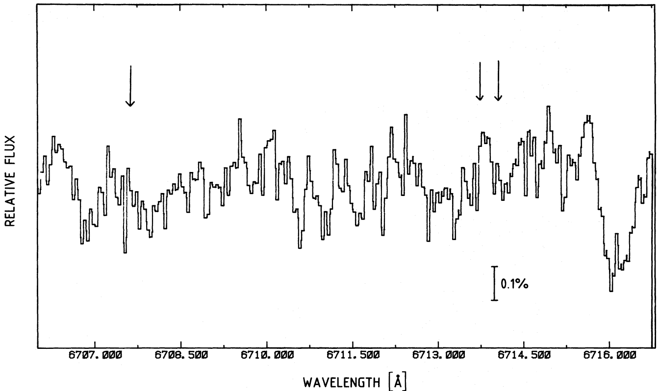
Fig. 1. The spectrum of SN 1987A around \lambda 6710 \text{ \AA} as observed with the CES, Short Camera, and CCD at a resolving power of \geq 60,000 ; a total of 15 spectra obtained at three different grating settings have been averaged. Note the high S/N per pixel but also the modulation at intermediate spatial wavelengths due to imperfectly flatfielded fringing effects in the CCD. Arrows indicate the positions of features attributed by Vidal-Madjar et al. (1987) to interstellar lithium. In order to facilitate the comparison, we have chosen the same scaling as in Vidal-Madjar et al.'s Fig. 2; the flux scale in units of the adjacent pseudo continuum is indicated by the vertical bar in the lower right corner
