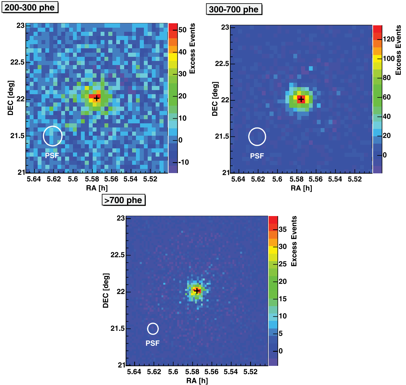
FIG. 15.—Sky maps of excess events from the Crab Nebula for different \gamma -ray energies ( \sim 160 , \sim 250 , and >500 GeV). The position of the pulsar is marked by the black plus sign, and the angular resolution is indicated by the circle.
