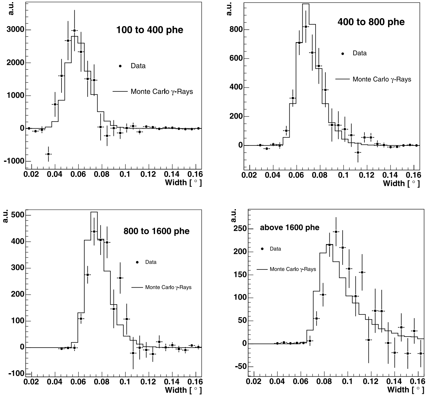
FIG. 3.—Distribution of the image parameter WIDTH for \gamma -ray events extracted from data and for MC simulated \gamma -rays in four consecutive bins of SIZE covering the full analyzed energy range.
