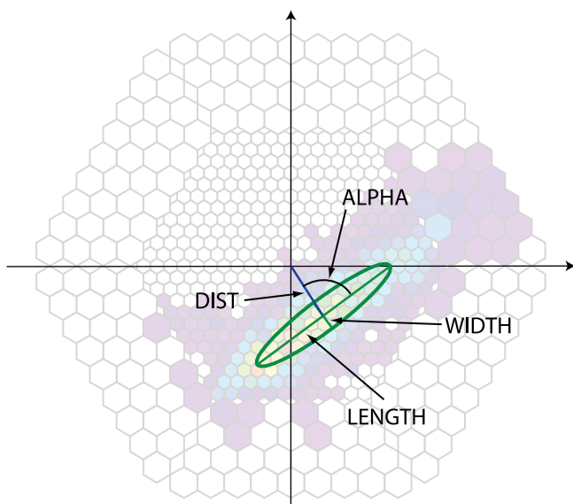
FIG. 1.—Parameterization of a shower image with Hillas parameters.
