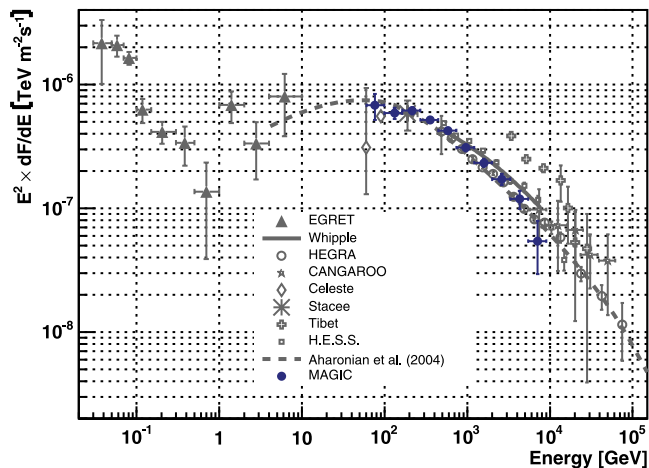
FIG. 11.—SED of the \gamma -ray emission of Crab Nebula. The measurements shown below 10 GeV are by EGRET (de Jager et al. 1996). In VHE \gamma -rays, measurements are from ground-based experiments. Above 400 GeV our measurement is in agreement with measurements by other IACTs. The dashed line is a model prediction by Aharonian et al. (2004).
