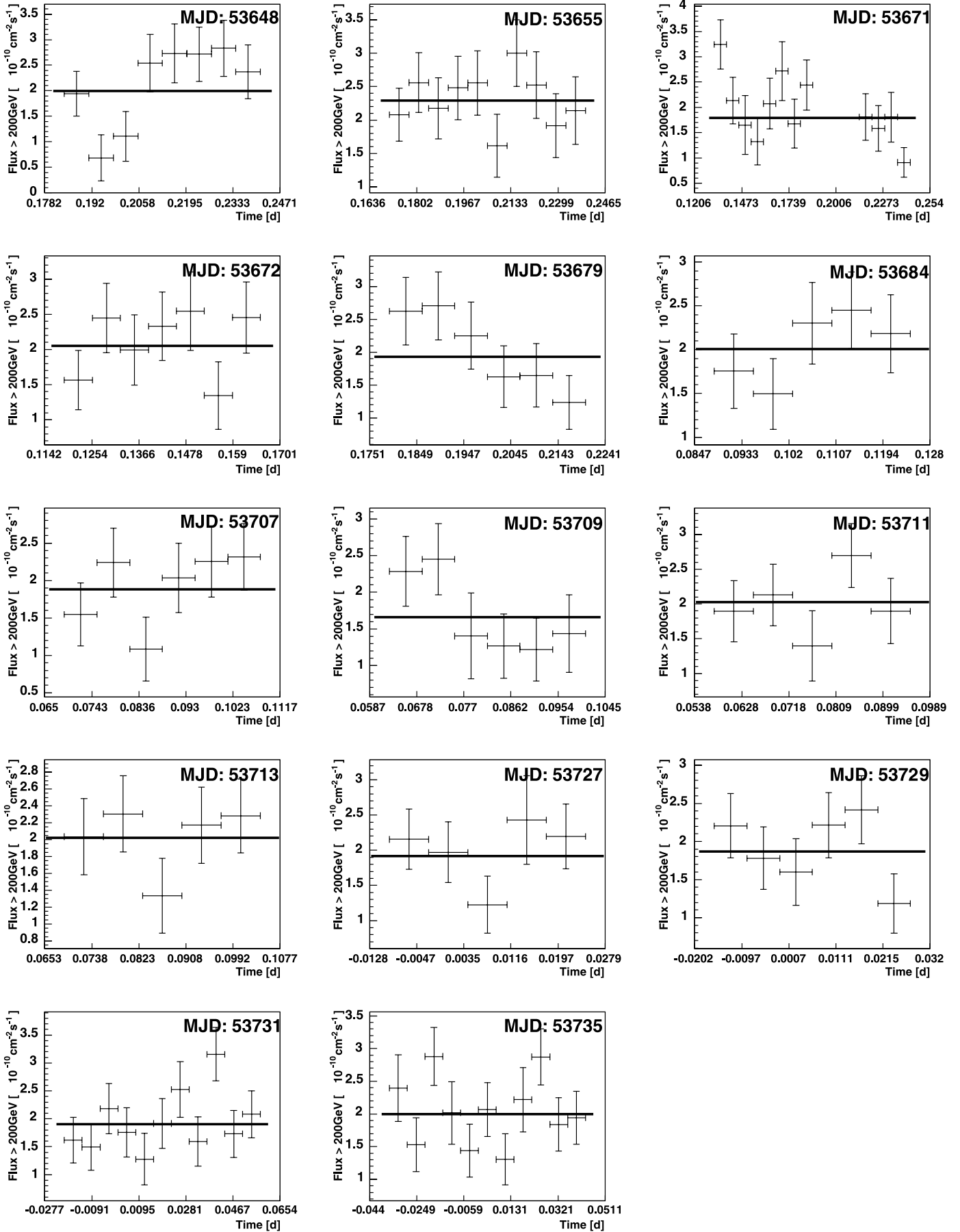
Fig. 13.—Light curves of the integral flux above 200 GeV from the Crab Nebula for each night.
