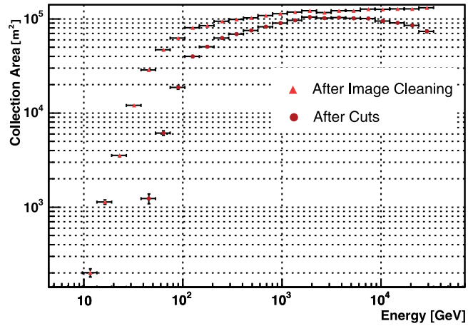
FIG. 9.—Collection area after image cleaning and after cuts for low zenith angle observations ( < 20^\circ ).
