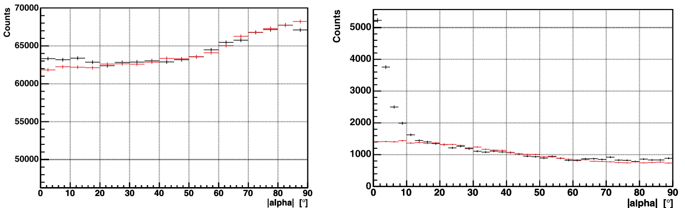
FIG. 5.—Distribution of the image parameter |\text{ALPHA}| for the bin of reconstructed energy 80–100 GeV in the left panel and for events with energies >200 GeV in the right panel. ( black : ON data; red : OFF data)
