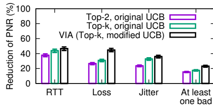
Figure 15: Comparing guided-exploration strategies.
