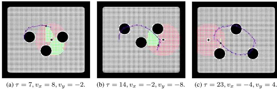
Fig. 11: 2D viability kernel slices of the unstopable pursuit scenario at different times.
