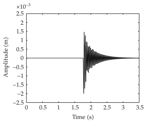
(e) Output measured along the x direction of the bearing B_3 .
