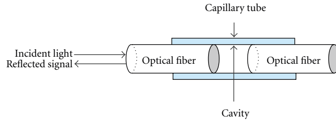
FIGURE 11: Extrinsic Fabry-Pérot interferometers, based in capillary tube.
