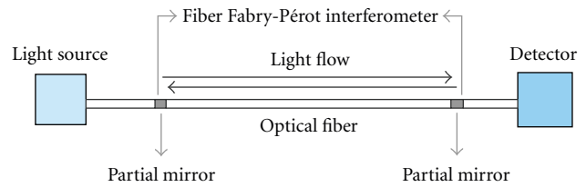
FIGURE 10: General structure of in-fiber Fabry-Pérot interferometers.
