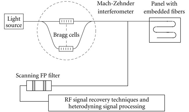
FIGURE 16: Schematic of high resolution vibration measurements using wavelength demultiplexed fiber Fabry-Pérot sensors.
