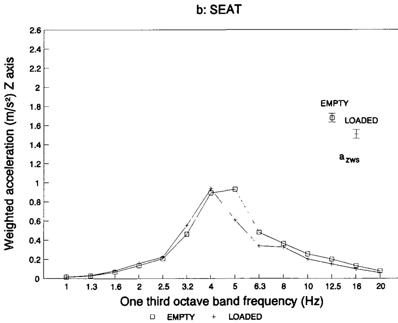
Fig. 1. Average one-third octave band spectra of the weighted equivalent acceleration on (a) the floor and (b) the seat, in the vertical axis, without and with a load.
