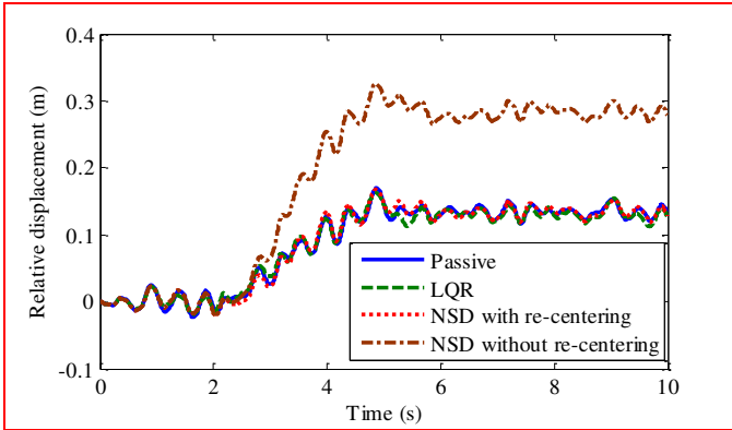
Fig. 15 Time history of relative displacement between the car body and lead bogie (LQR: \mathbf{R}=\mathbf{I}\times 10^{-6} , NSD: k_n = -210 kN/m)
