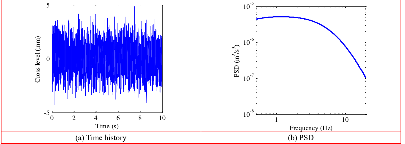
Fig. 3 Cross level of track irregularity
