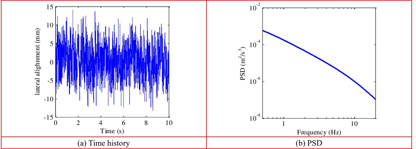
Fig. 2 Lateral alignment of track irregularity
