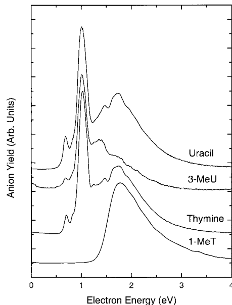
FIG. 4. Negative ion yield as a function of electron energy in uracil, 3-methyluracil, thymine, and 1-methylthymine.
