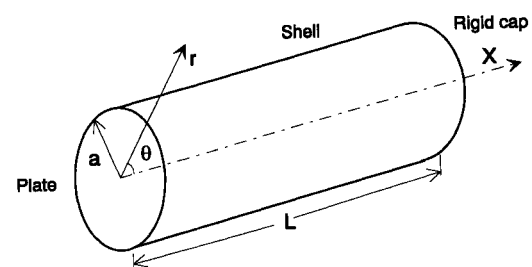
FIGURE 2 Schematic diagram of the structure under investigation.
