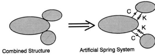
FIGURE 3 Schematic representation of the coupling modeling using the artificial spring system.
