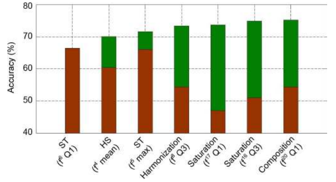
Fig. 11. The performance comparison of the SBFs chosen in AFSim (the green bar) and that of the individual SBF (the brown bar) are plotted. Y-axis indicates the VAQ performance in accuracy. The brown bar in x-axis demonstrates the accuracies of the used features respectively and the green bar shows the accuracies of the features added from left to right. From this result, it clearly shows that forward-selection procedure (the green bar) can enhance the accuracy consistently by selecting useful video-based features, regardless of the individual feature performance (the brown bar) being limited.
