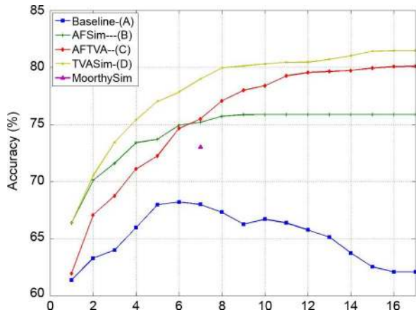
Fig. 12. The accuracies of Baseline, AFSim, AFTVA, TVASim, and MoorthySim obtained by varying the number of the SBFs selected. The x-axis represents the number, and the y-axis indicates the corresponding accuracy.
