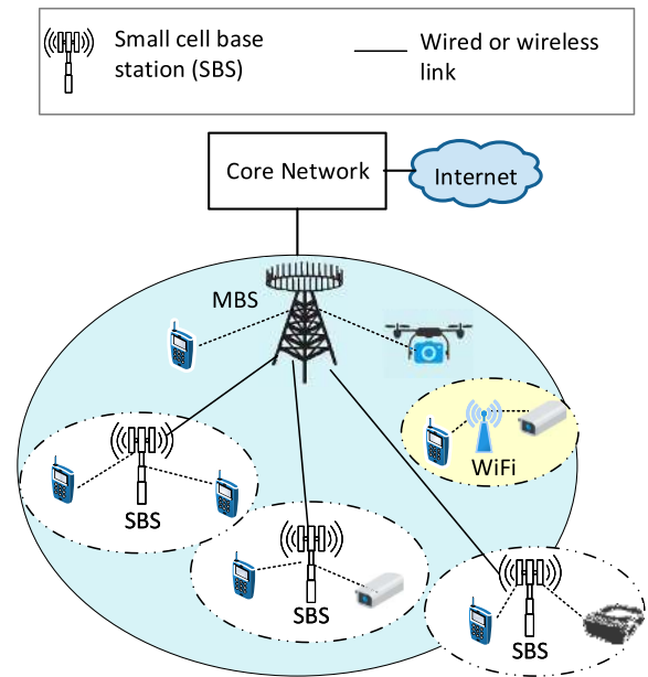
Fig. 10. HetNet architecture.
