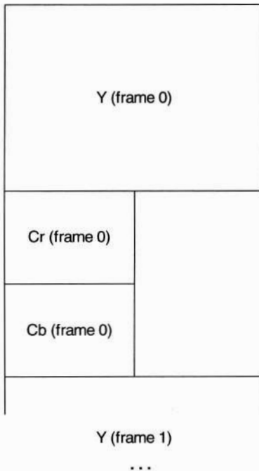
Figure 13.3 YV12 (4:2:0)
