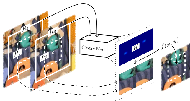
Figure 1: Pixel interpolation by convolution. For each output pixel (x, y) , our method estimates a convolution kernel K and uses it to convolve with patches P_1 and P_2 centered at (x, y) in the input frames to produce its color \hat{I}(x, y) .
