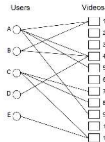
Figure 2: User-Video Graph. An alternate way of representing the co-view information is implicitly through the user-video bipartite graph. The number of co-views is computed by examining the number of paths of length 2 that exist between any two videos.
