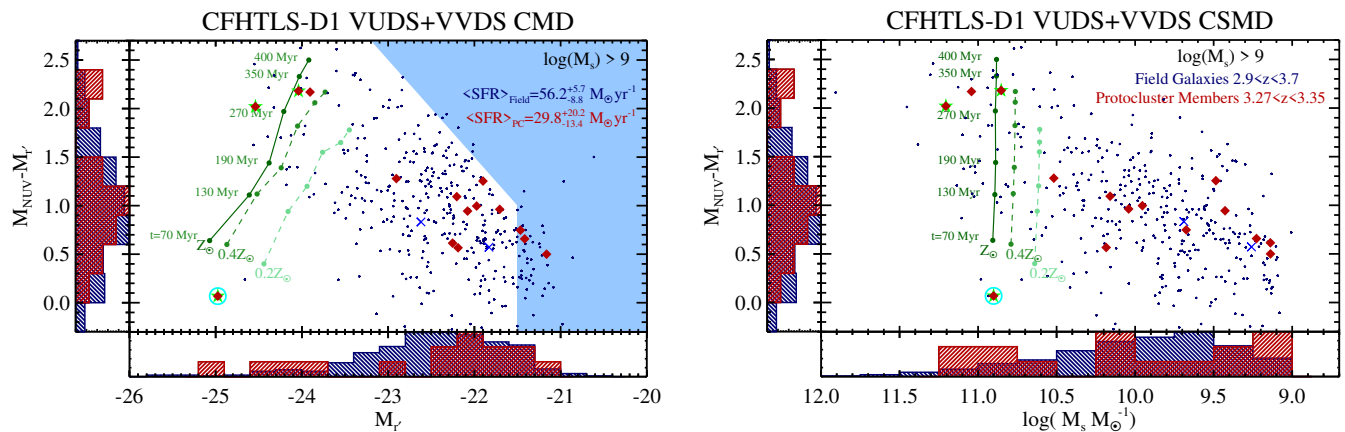
Fig. 10. Left: Rest-frame M_r/M_{NUV} - M_r CMD of all galaxies in the entire CFHTLS-D1 field with secure redshifts 2.9 < z_{spec} < 3.7 and stellar masses \log(M_s) > 9 . The stellar mass cut is imposed here in an attempt to mitigate any induced differential bias between the field and protocluster members (see §4.1.2). The meanings of the symbols are identical to those of Figure 9 as is the meaning of the light blue-shaded region and the galaxy model tracks. Here and in the right panel, color and absolute magnitude histograms, normalized such that the maximum value is unity, are shown for each population. While most protocluster members have relatively typical colors and magnitudes with respect to the field, there exists a sub-dominant population of extremely bright (and typically redder) protocluster galaxies. The median SFRs, as derived from the SED fitting process, of the two samples is shown in the upper right hand corner. Right: Color-stellar-mass (CSMD) of the same galaxy populations shown in the left panel. The meanings of all symbols are the same. The bimodality observed in the CMD remains in the CSMD, with several protocluster galaxies having with extreme stellar masses \log(M_s) \gtrsim 10.8 . These galaxies comprise some of the most massive galaxies in the entire spectroscopic sample in the range 2.9 < z_{spec} < 3.7 . Though several field galaxies exhibit similar colors and stellar masses, the volume used to define the field sample is \sim 250 larger than that used to define the bounds of the protocluster. The proto-BCG, marked by the circumscribed cyan circle, likely has its stellar mass estimate contaminated by the presence of its powerful AGN, though the other two type-1 AGN hosts likely do not.
