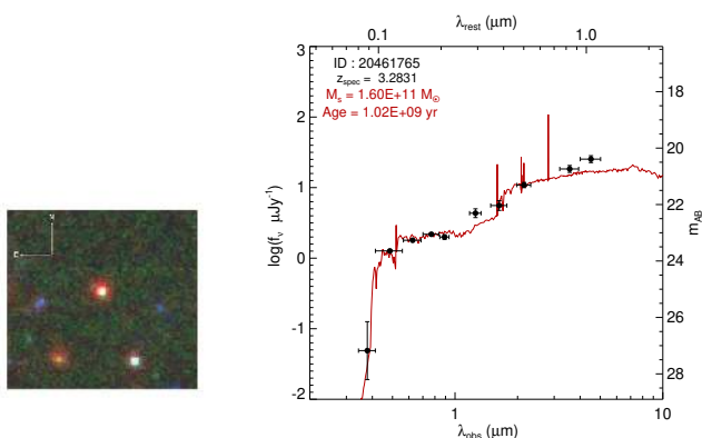
Fig. 12. Left: Postage stamp of the most massive galaxy in Cl J0227-0421 generated in an identical manner to that of Figure 11. Right: Observed-frame optical/NIR SED of this galaxy plotted against the best-fit galaxy template. As before, the best-fit stellar mass and luminosity-weighted stellar age are shown in the upper left corner of the plot. While this galaxy is also host to a type-1 AGN, the properties of its SED are much different than that of the proto-BCG and the SED is generally well fit by the galaxy template. There is some discrepancy in the IR portion of the SED, but an identical stellar mass is recovered (within the random errors) if IRAC bands are excluded from the fit.
