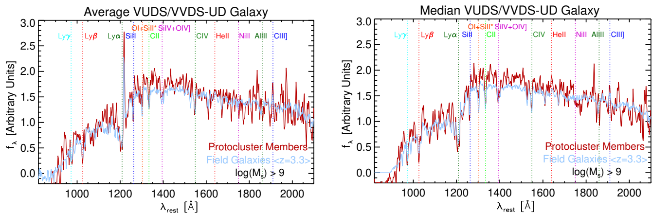
Fig. 15. Left: Rest-frame mean “coadded” VUDS spectra of all spectral members of Cl J0227-0421 with \log(M_*) > 9 plotted against that of the field galaxy sample. All type-1 AGN hosts are removed from both samples. Important spectral features are noted. The two spectra exhibit remarkably similar properties. Subtle differences do exist; the average protocluster galaxy appears to have slightly stronger emission features ( \text{Ly}\alpha , HeII, and CIII]) and a steeper rest-frame NUV continuum slope. Right: Median “coadded” VUDS spectra of the same two samples shown in the left panel. The major difference between the median spectra and the mean spectra plotted in the left panel is the enormous decrease in the strength of the \text{Ly}\alpha line, which is a reflection of the fact that most galaxies do not emit \text{Ly}\alpha at these redshifts. In the median spectrum, the \text{Ly}\alpha emission is roughly equivalent among the field galaxies and the protocluster members, owing to the similar fractional contribution of LAEs to both samples (see text). The differences in the median and mean spectra suggest that, though the galaxies in the protocluster emit \text{Ly}\alpha roughly as frequently as the general field population, those galaxies which do emit \text{Ly}\alpha in the protocluster are doing so more profusely.
