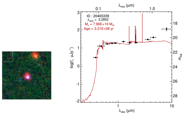
Fig. 11. Left: Postage stamp of the X-ray and type-1 AGN host proto-BCG of Cl J0227-0421. Blue, green, and red channels are assigned to the i'K_s[4.5] bands, respectively, and logarithmic scaling is used for the brightness. Image dimensions are 25'' ( \sim 200 kpc at z \sim 3.3 ) on each side. The bright object to the north-northwest of the proto-BCG was not targeted by spectroscopy, but has a well-fit photometric redshift of z_{phot} = 1.21 \pm 0.03 . Right: Observed-frame optical/NIR spectral energy distribution (SED) of the proto-BCG with the best-fit galaxy template overplotted in red. The proto-BCG has a power-law continuum both in the UV and in the IR, suggesting the physical parameter estimates coming from the SED fitting process are contaminated by the presence of the AGN. The best-fit stellar mass and luminosity-weighted stellar age are shown in the upper left corner of the plot.
