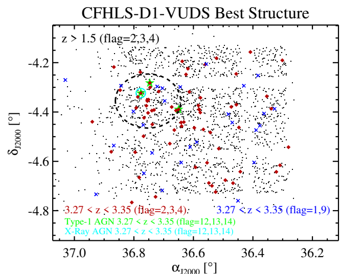
Fig. 3. Sky distribution of galaxies in the redshift range of the most significantly detected spectroscopic protostructure in the CFHTLS-D1 field (CI J0227-0421). Galaxies with secure spectroscopic redshifts are plotted as red diamonds, those with less secure spectroscopic redshifts are shown as blue Xs. Green stars denote those galaxies hosting a type-1 AGN and the cyan circle denotes the lone X-ray AGN host at these redshifts. Plotted in the background are all galaxies in the CFHTLS-D1 field with secure spectroscopic redshifts z_{\text{spec}} > 1.5 . The dashed circle designates 3 h_{70}^{-1} Mpc from the adopted center of the protostructure and is used in conjunction with the redshift range to define membership (see §3.1). The VIMOS footprint is clearly visible, and coverage gaps in the CFHTLS-D1 spectroscopy are apparent throughout the field and to the north of the protostructure.
