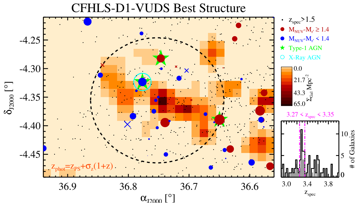
Fig. 4. Left: Zoom-in of the sky distribution of all galaxies in the redshift range of the same protostructure that is shown in Figure 3 (CI J0227-0421). This protostructure is also the most significantly detected protostructure in photometric redshift overdensity. The photometric density map, generated using the methodology of §3, is shown in the background, with the scale bar denoting the photometric redshift galaxy density. As in Figure 3, the dashed circle designates 3 h_{70}^{-1} Mpc from the adopted center of the protostructure. Blue and red symbols show galaxies at the redshift of the protostructure differentiated by their M_{NUV} - M_r colors (where the delineation point was set roughly at the color of a 200 Myr old stellar population, see §4.1.2) and are logarithmically scaled ( \log_4 ) by their stellar mass (see §4.1). Filled circles denote galaxies with secure spectroscopic redshifts, while Xs denote those galaxies with less secure spectroscopic redshifts. Plotted in the background are all galaxies with z_{spec} > 1.5 . Several massive, redder galaxies are observed in the bounds of the protostructure and extended filamentary structure can be seen to the west-southwest of the central protostructure galaxy concentration. Bottom right: Spectroscopic redshift distribution of galaxies within 3 h_{70}^{-1} Mpc of the protostructure center. The shaded histogram displays only those galaxies with secure spectroscopic redshifts, while the histogram plotted with a solid black line also includes those galaxies with less secure spectral redshifts. The redshift bounds defining membership are marked by magenta dot-dashed lines.
