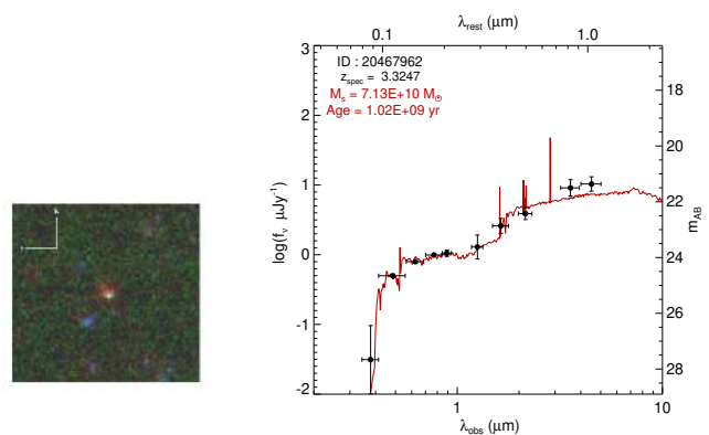
Fig. 13. Left: Postage stamp of the third brightest and fourth most massive galaxy in Cl J0227-0421 generated in an identical manner to that of Figure 11. Right: Observed-frame optical/NIR SED of this galaxy plotted against the best-fit galaxy template. Best-fit stellar mass and luminosity-weighted stellar age are shown in the upper left corner of the plot. While this galaxy is also host to a type-1 AGN, the same test was performed on this galaxy as was performed on the galaxy shown in Figure 12 and negligible differences in the derived stellar mass were found.
