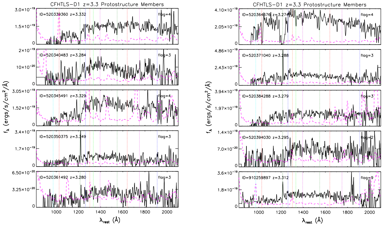
Fig. 7. Mosaic of the one-dimensional rest-frame VIMOS spectra remaining nine spectral members of CI J0227-0421. Also plotted in the bottom right hand panel (ID=910259897) is the only member with a less secure spectroscopic redshift that exhibits a strong emission line in its spectrum. In this case we presume the line to be Ly \alpha , though this galaxy does not enter any of our analysis and is presented here and elsewhere only for illustrative purposes. The meanings of all lines are the same as in Figure 6.
