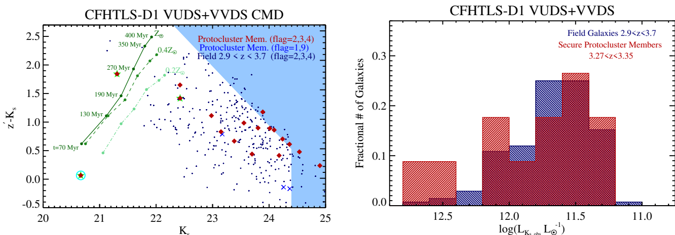
Fig. 9. Left: Observed-frame CFHTLS/WIRDS color-magnitude diagram (CMD). Members of CI J0227-0421 with secure spectroscopic redshifts are shown as red diamonds, those with less secure spectroscopic redshifts are shown as blue Xs. The meanings of the green star and cyan circle are the same as those in Figure 3. All galaxies in the entire CFHTLS-D1 field with secure spectroscopic redshifts 2.9 < z_{spec} < 3.7 that do not reside in the bounds of CI J0227-0421 (i.e., “field galaxies”, see §4.1) are plotted as small navy points. The light blue-shaded region indicates the region of this phase space not probed to the 5\sigma point-source completeness limits of the CFHTLS/WIRDS imaging. Model tracks for a z = 3.3 L^* galaxy with three different stellar metallicities are overplotted (see §4.1.2). Several galaxies which are extremely bright in the K_s band, including two of the four brightest galaxies in the entire spectroscopic sample over this redshift range, are members of the protocluster. Right: Fractional distribution of observed-frame K_s -band luminosities in the protocluster and field samples. Only those protocluster members with secure spectroscopic redshifts and only those galaxies lying outside of the blue shaded region in the left panel are plotted. Though a large fraction of the protocluster member galaxies have relatively normal K_s -band luminosities with respect to the general field population, the percentage of bright ( \log(L_{K_s}) \gtrsim 12.0 ) galaxies residing in CI J0227-0421 is nearly double that of the field.
