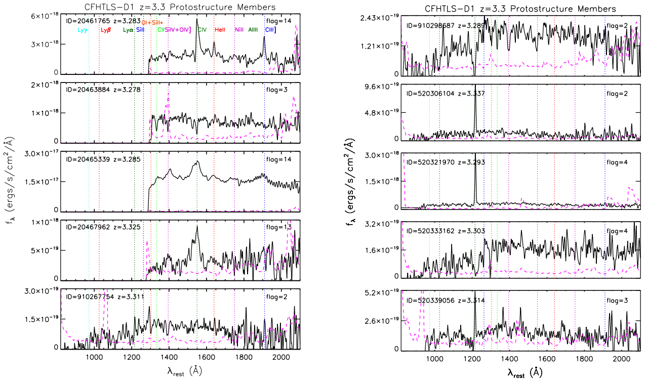
Fig. 6. Mosaic of the one-dimensional rest-frame VIMOS spectra of ten spectral members of CI J0227-0421. The black line in each panel is the flux density spectrum, and the dashed magenta line is the formal uncertainty spectrum (see Le Fèvre et al. 2014 and references therein for details on the generation of the uncertainty spectrum). Important spectral features are marked. The spectrum of the proto-BCG, a type-1, and X-ray AGN host is shown in the 3rd panel from the top on the left. The spectra of the two other type-1 AGN hosts are shown in the top and 4th from the top panel on the left. The first four galaxies plotted in the left panel were observed as part of the VVDS-Deep sample and, as such, do not have observed spectra blueward of \lambda_{rest} \lesssim 1290\text{\AA} . A wide range of diversity in spectral properties is seen among the protostructure members.
