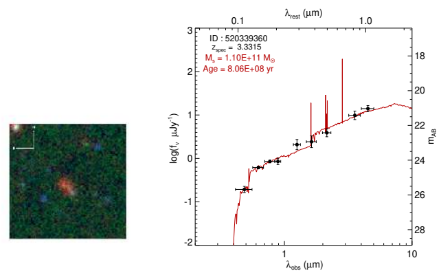
Fig. 14. Left: Postage stamp of the fourth brightest and second most massive galaxy in Cl J0227-0421 generated in an identical manner to Figure 11. Right: Observed-frame optical/NIR SED of this galaxy plotted against the best-fit galaxy template. Best-fit stellar mass and luminosity-weighted stellar age are shown in the upper left corner of the plot. This galaxy is not host to a type-1 AGN. Though the best-fit galaxy template appears significantly different from the other two massive, redder protocluster galaxies plotted in Figures 12 and 13, the dominant stellar population in this galaxy appears relatively old.
