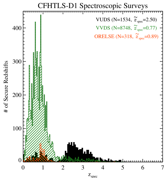
Fig. 1. Spectroscopic redshift distribution of the 10600 unique objects with secure spectroscopic redshifts (see text) in the CFHTLS-D1 field. The two lower redshift surveys, VVDS (Le Fèvre et al. 2013) and ORELSE (Lubin et al. 2009), are shown as hashed green and orange histograms, respectively. The higher redshift VUDS (Le Fèvre et al. 2014) objects are shown as a black filled histogram. The number of objects with secure spectroscopic redshifts coming from each survey along with the median z_{spec} of each sample is shown in the top right corner. For the sake of clarity, the bin size of the histograms for the VUDS and ORELSE objects are twice that of the VVDS. Though it is not apparent from the diagram, there is a tail of galaxies with z_{spec} > 5 confirmed from the VUDS survey.
