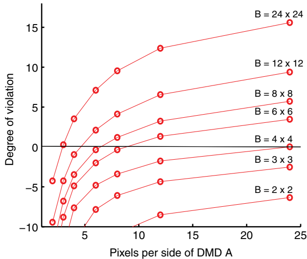
FIG. 1 (color online). Violation of our EPR steering inequality (2) for measurements of party B conditioned on measurements of party A as measured in standard deviations of the difference between the bound and the sum of conditional entropies. This plot was formed by independently downsampling the joint distributions for a 24 \times 24 data set. A positive value represents a violation. We see that below 4 \times 4 resolution for party B as suggested by theory, the inequality is not violated for any resolution of DMD A , but violation is possible for large resolution of party B and party A having resolution below 4 \times 4 .
