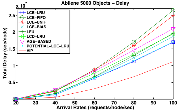
Figure 3: Abilene Network: Delay
