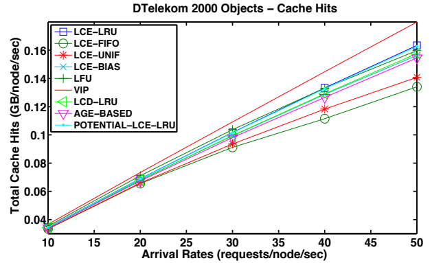
Figure 10: DTelekom Network: Cache Hits
