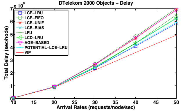
Figure 6: DTelekom Network: Delay
