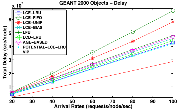
Figure 4: GEANT Network: Delay
