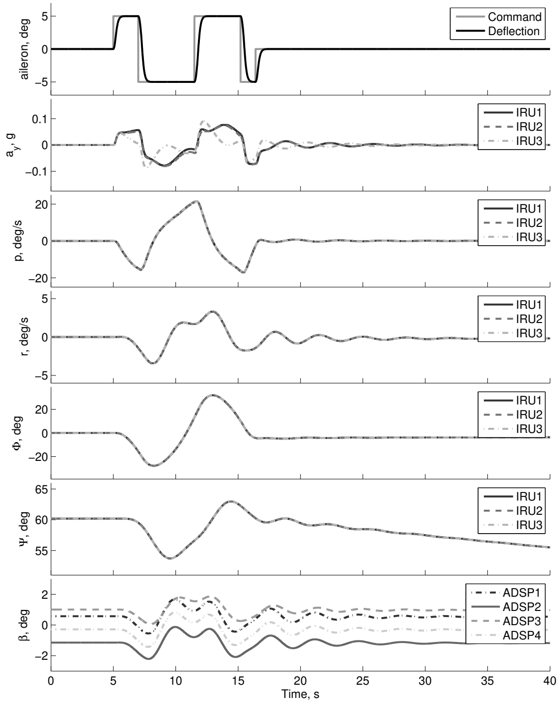
Fig. 4 Response of the VIRTAC-Castor model to an aileron input
