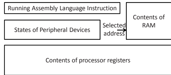
Fig. 8 Simulation of functionality of an 8-bit processor
